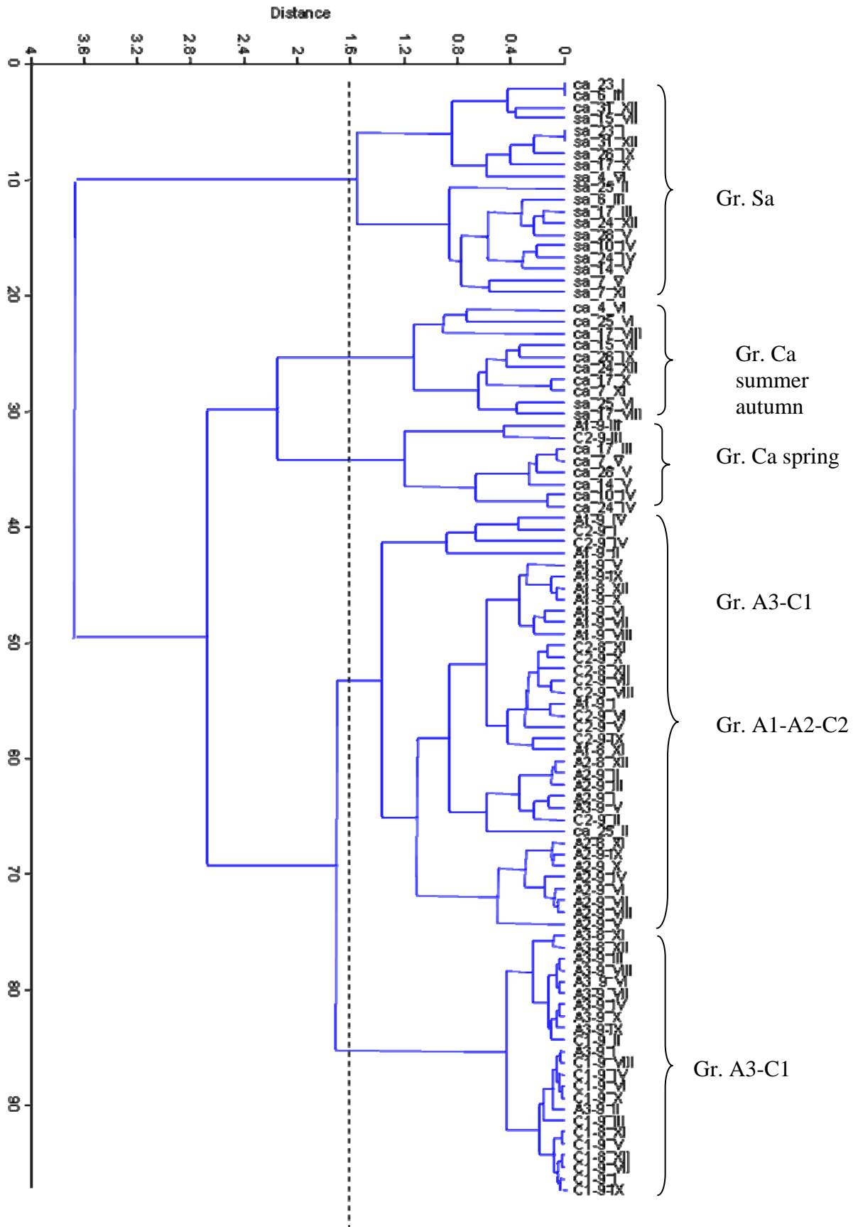
Appendix III. CAH of the 3 first axes of CA. The vertical truncature line is dotted.
