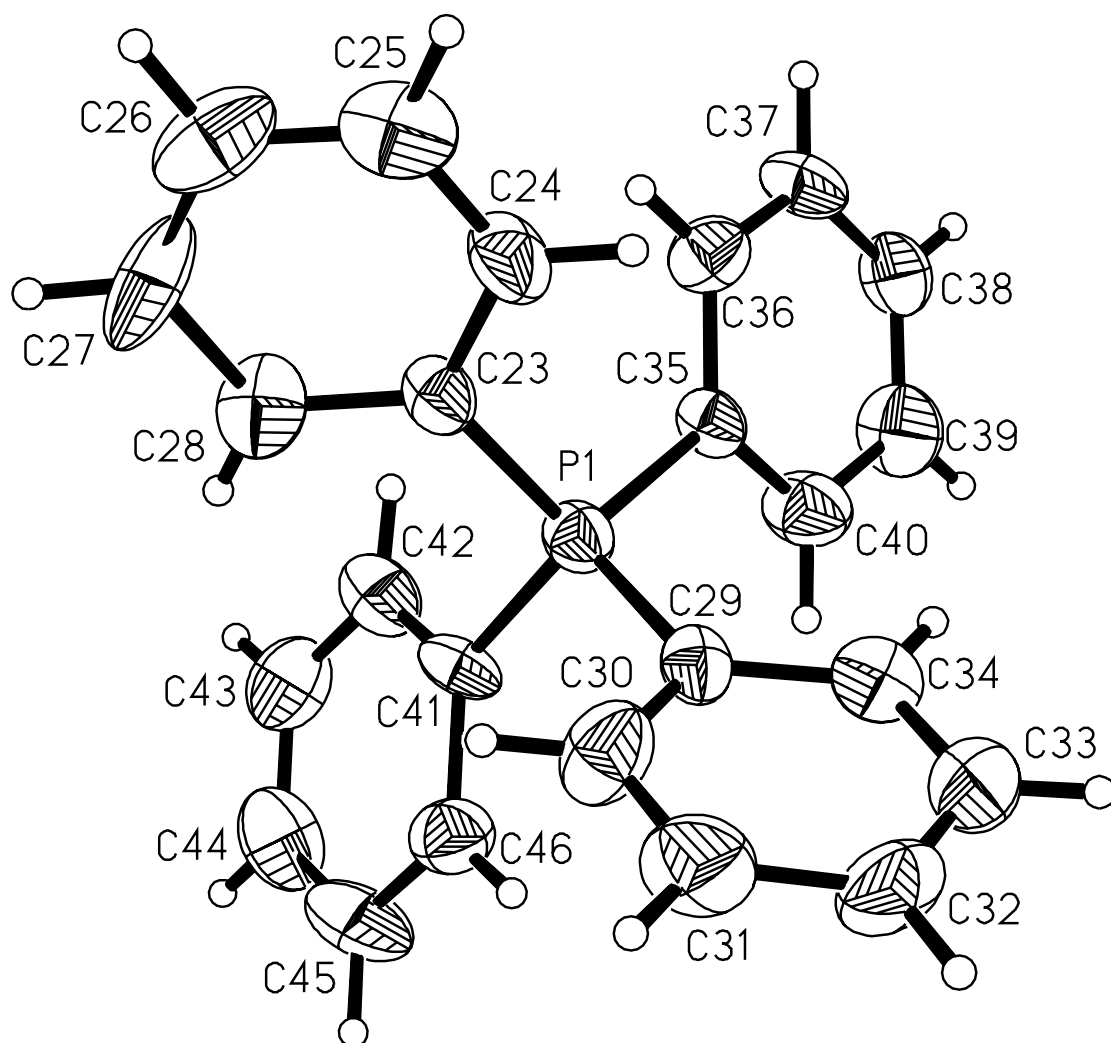
Figure S1. Atomic numbering scheme of the \text{PPh}_4^+ cation associated with phosphorous atom P1 in the (\text{PPh}_4)_3[\text{Cu}_4(\text{dca})_{11}] salt. Thermal ellipsoids are drawn at the 50% probability level.
