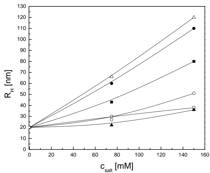
Figure S3: The effect of various cations / chloride salts on the growth of the hydrodynamic radii R_H of the cationic aggregates in SL / DTAB systems: NaOAc (▲), \text{Na}_2\text{SO}_4 (□), NaCl (○), \text{NaNO}_3 (■), NaBr (●) and NaSCN (Δ).
