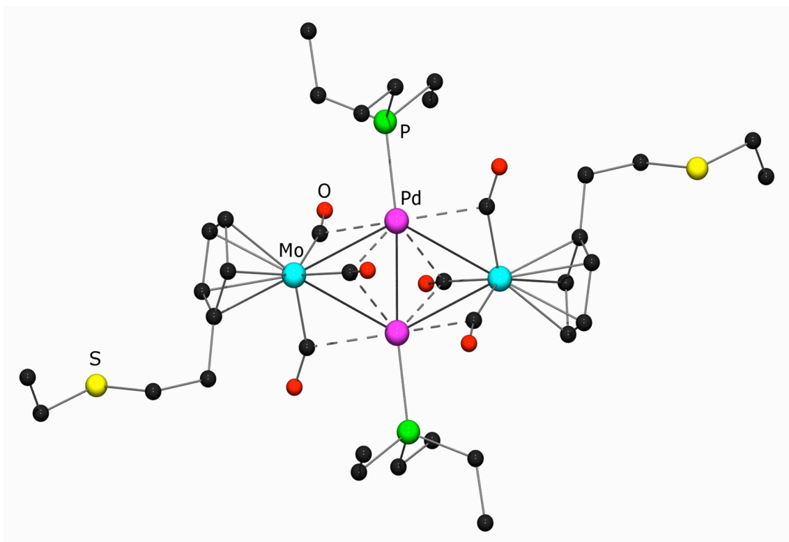
Figure 1b. View of the crystal structure of 5
