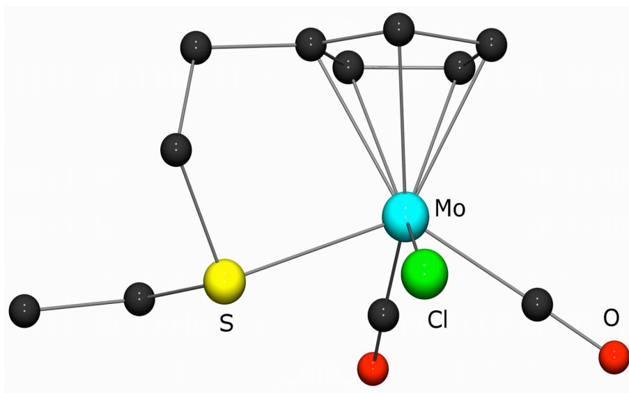
Figure 4b. View of the crystal structure of 8
