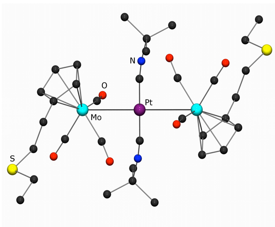
Figure 2b. View of the crystal structure of 6
