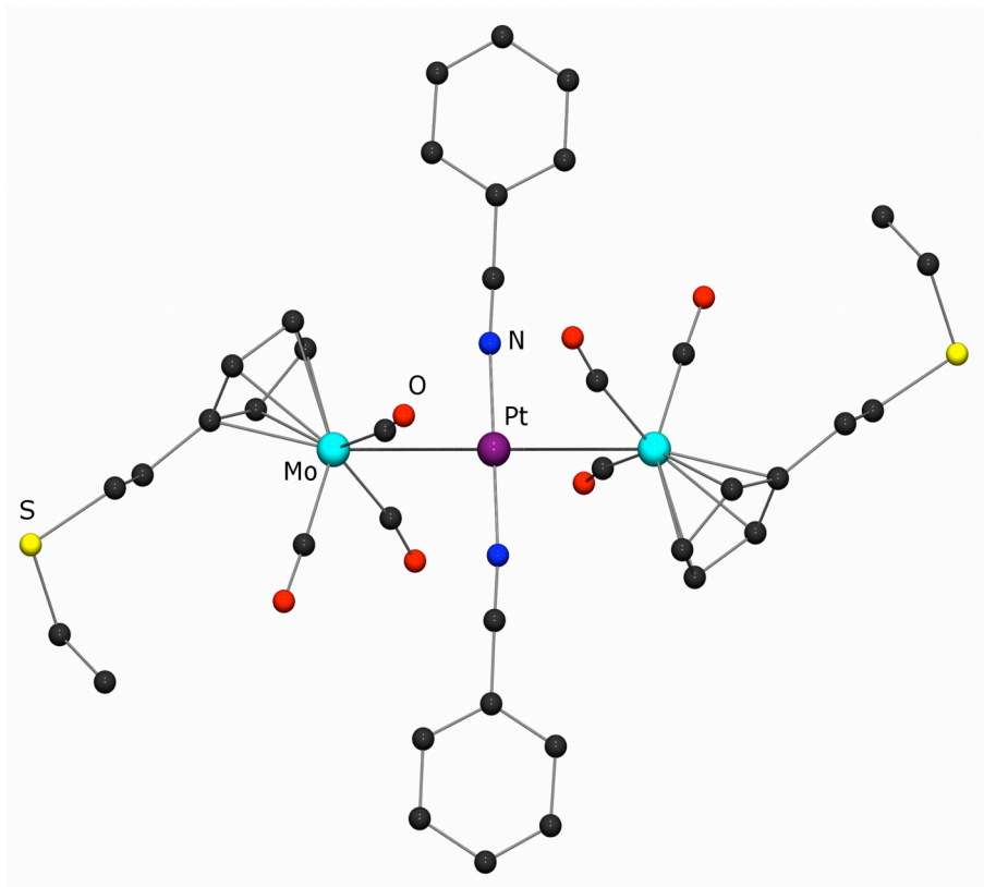
Figure 3b. View of the crystal structure of 7
