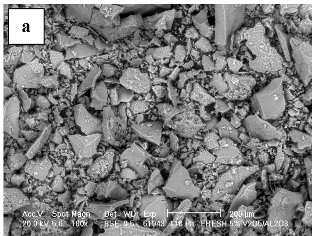
Fig. S1. SEM micrographs of the vanadium-containing samples before and after the catalytic test: (a) – fresh 5V-Al 2 O 3 ; (b) – used 5V-Al 2 O 3 ; (c) – fresh 10V-Al 2 O 3 ; (d) – used 10V-Al 2 O 3 .
