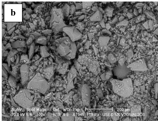
Fig. S1. SEM micrographs of the vanadium-containing samples before and after the catalytic test: (a) – fresh 5V-Al 2 O 3 ; (b) – used 5V-Al 2 O 3 ; (c) – fresh 10V-Al 2 O 3 ; (d) – used 10V-Al 2 O 3 .
