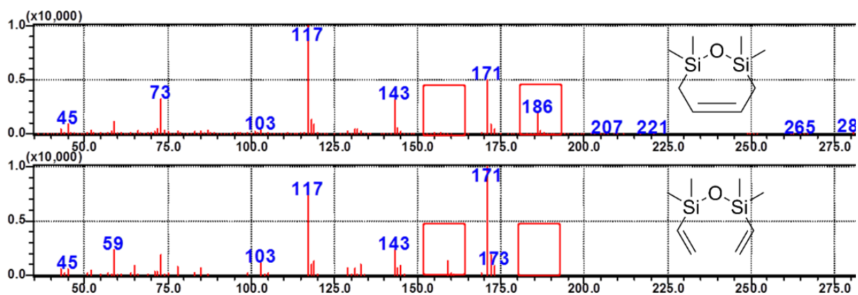
Figure S2 Compounds 24 and 25 spectra comparison
