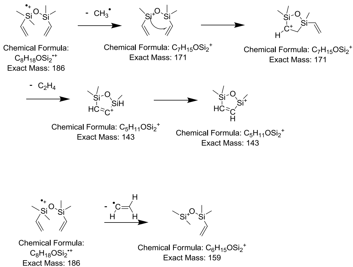
Figure S4 Fragmentation process of compound 25
