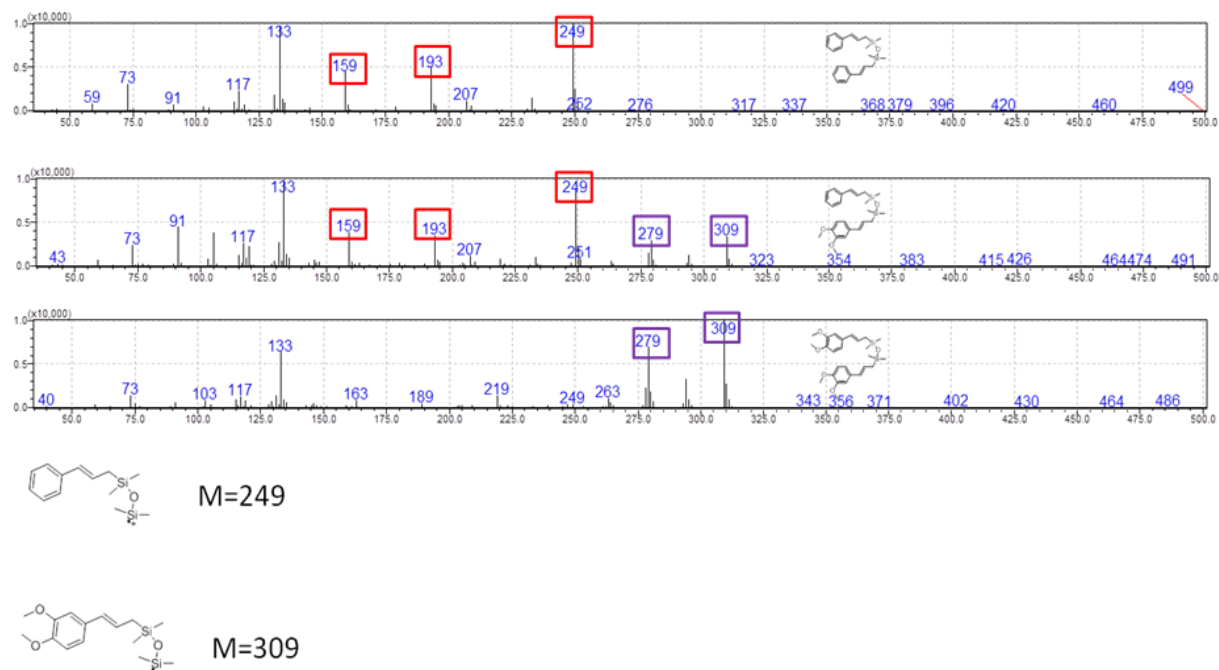
Figure S1 MS spectra of compounds 12,15 and 23
