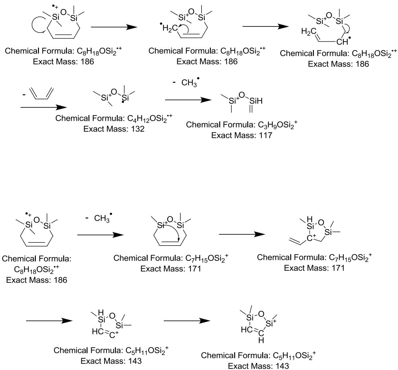
Figure S3 Fragmentation process of compound 25
