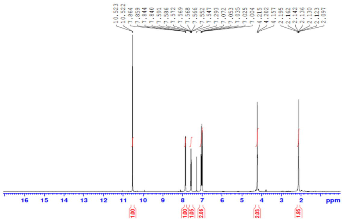
Figure S1. The ^1\text{H} NMR of 1,4-bis(2-carboxyaldehyde phenoxy)butane in \text{CDCl}_3
