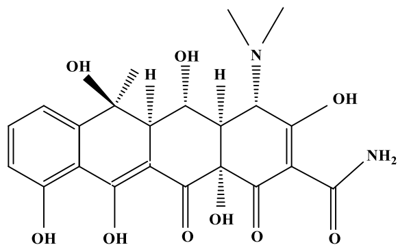
Supplementary Figure S1. Structural scheme of OTC ( C_{22}H_{24}N_2O_9 ).
