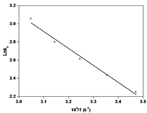
Supplementary Figure S2. Equilibrium constant versus the reciprocal of the temperature.
