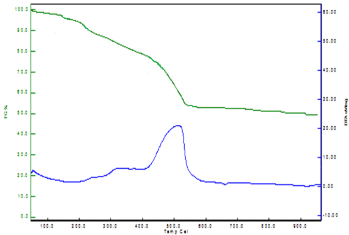
Fig. 7. TG-DTA graph of the Pt (II) complex
