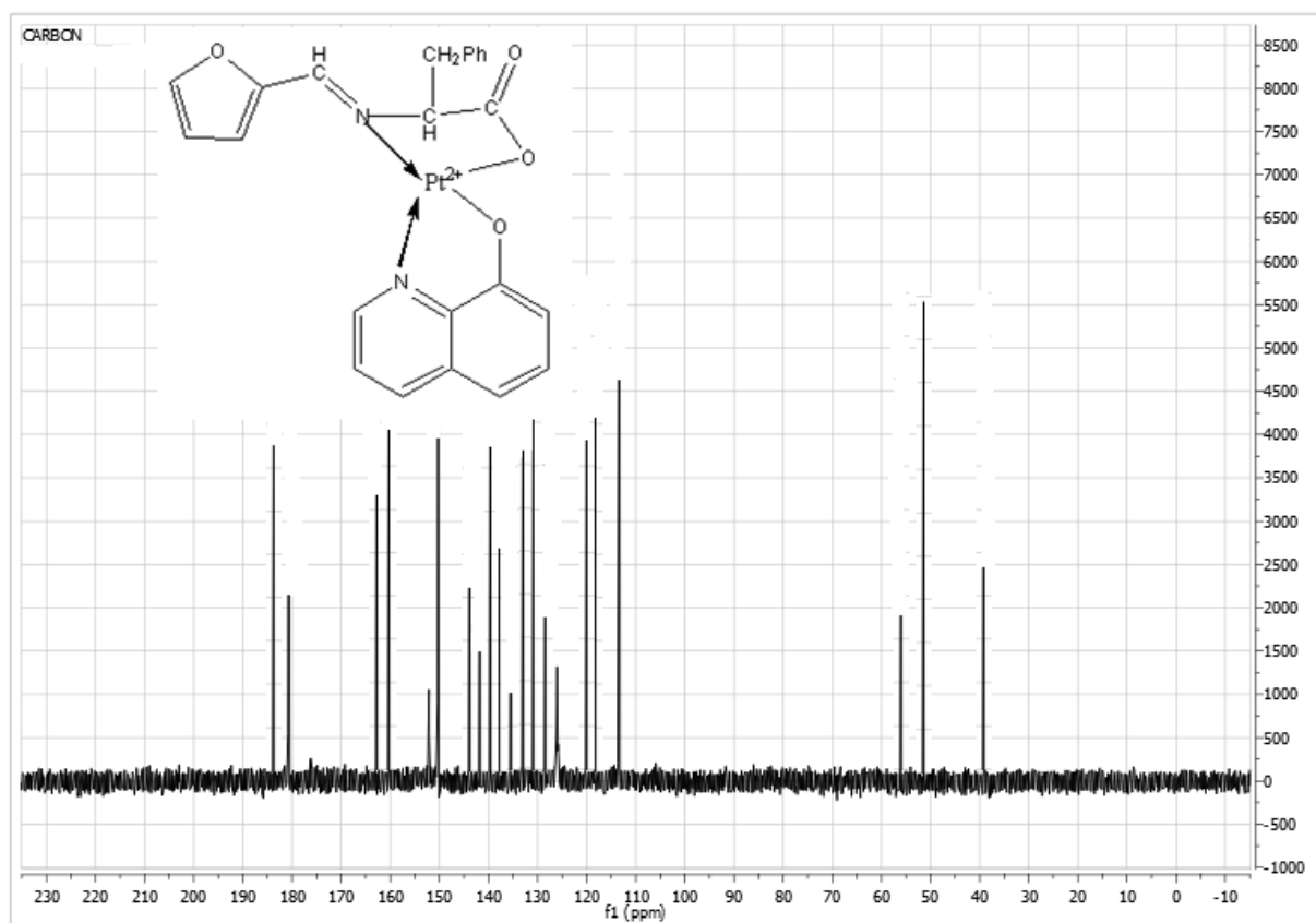
Fig. 6. ^{13}\text{C} NMR spectrum of the Pt (II) complex
