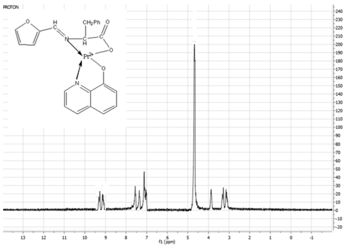
Fig. 4. ^1\text{H} NMR spectrum of the Pt (II) complex
