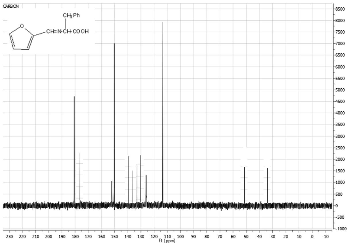
Fig. 5. ^{13}\text{C} NMR spectrum of the L^1
