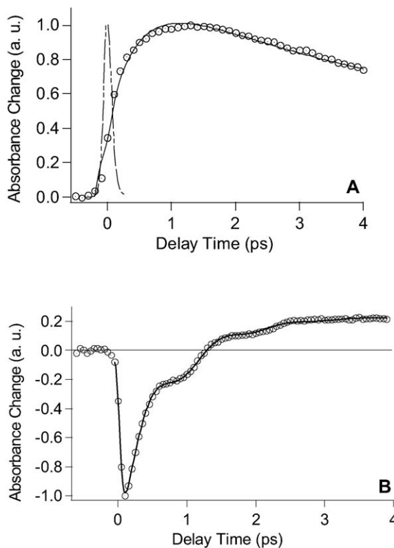
Fig. 2. A. Transient absorption data after pumping at 500 nm and probing at 625 nm for pump fluence of 500 nJ per pulse for gold NPs. The dashed line represents the pump-probe cross correlation of the instrument. B. Transient absorption data after pumping at 525 nm and probing at 600 nm for pump intensity at 675 nJ per pulse. The solid lines in Fig. 2A and B are fits of the experimental data according to equations (1) and (2), respectively.
