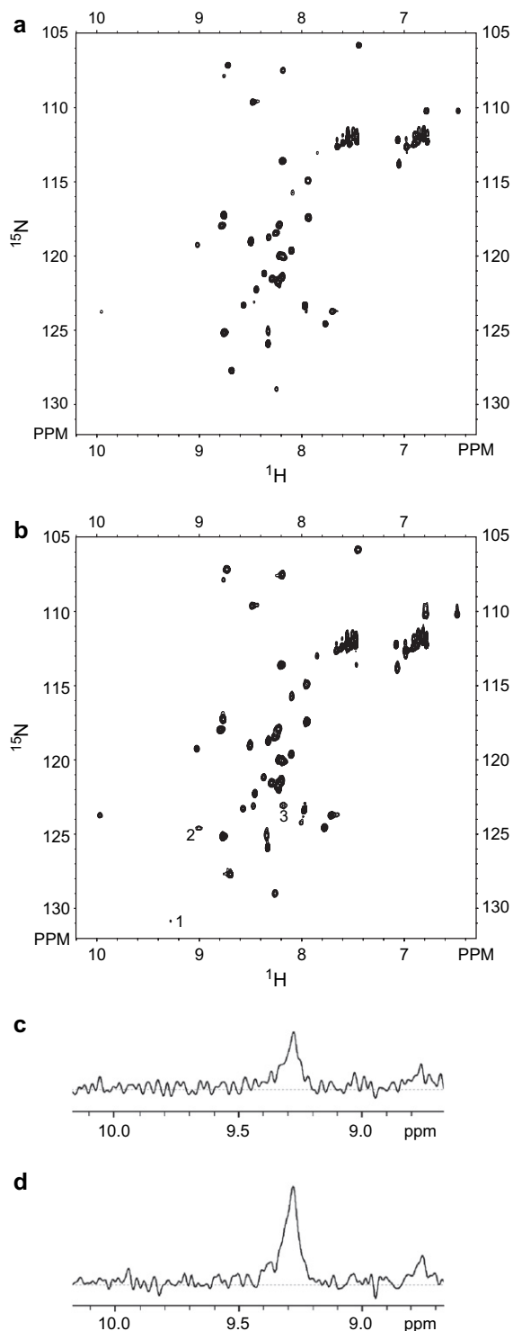
Fig. 2. Contour plot of the 2D HSQC-type spectra of the complex between uniformly 15 N-labelled NC and (a) unlabelled tRNA Lys 3 D-arm (SE-HSQC experiment), (b) unlabelled tRNA Lys 3 D-arm (SE-CPMG-HSQC experiment), (c) 1D SE-HSQC trace of signal 1 and (d) 1D SE-CPMG-HSQC trace of signal 1.
