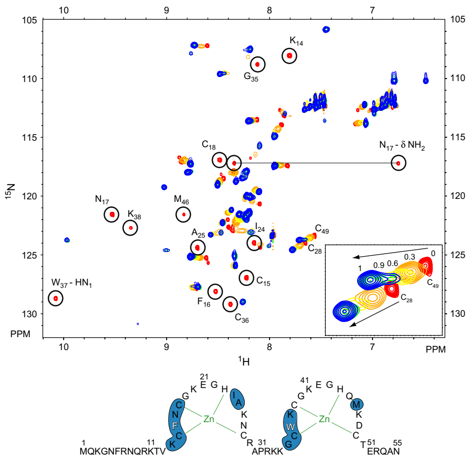
Fig. 3. Titration experiment (SE-CPMG-HSQC) of ^{15}\text{N} -labelled NC protein by unlabelled \text{tRNA}_{3^{\text{Lys}}} D hairpin. In red: 1/0 protein/RNA ratio; in orange: 1/0.3; in yellow: 1/0.6, in green: 1/0.9, in blue: 1/1. (For interpretation of the references to colour in this figure legend, the reader is referred to the web version of this article.) The circled signals disappear during the titration. The corresponding residues are highlighted on the NC sequence. The major aromatic residue of each zinc knuckle is written in open letter.
