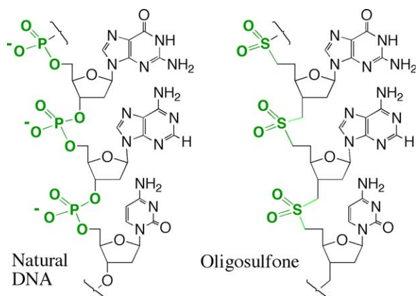
Fig. 5. Replacing phosphates ( -\text{PO}_2^- units, each having a negative charge, left) in DNA by dimethylenesulfone linkers (the -\text{SO}_2^- units, right, each lacking a negative charge) gave an uncharged analog of DNA. The uncharged analog of RNA was also synthesized.
