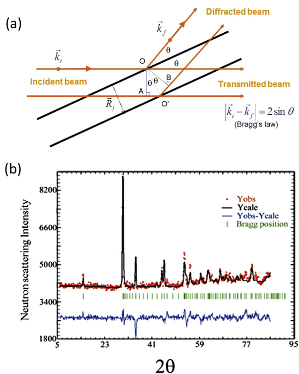
Fig. 2. (a) Schematic representation of the Bragg law in diffraction, 2d_{hkl} \sin \theta = \lambda , relating the diffraction angle \theta , the beam wavelength \lambda , and the space between lattice planes (in thick dark lines) d_{hkl} . (b) Rietveld refinement result of the NPD diagram of a cystine kidney stone (experimental data Y_{obs} in red, calculated profile Y_{calc} in black, and Y_{obs} - Y_{calc} difference in blue). Tick marks in green below the profiles indicate the peak positions of allowed Bragg reflections for cystine.
