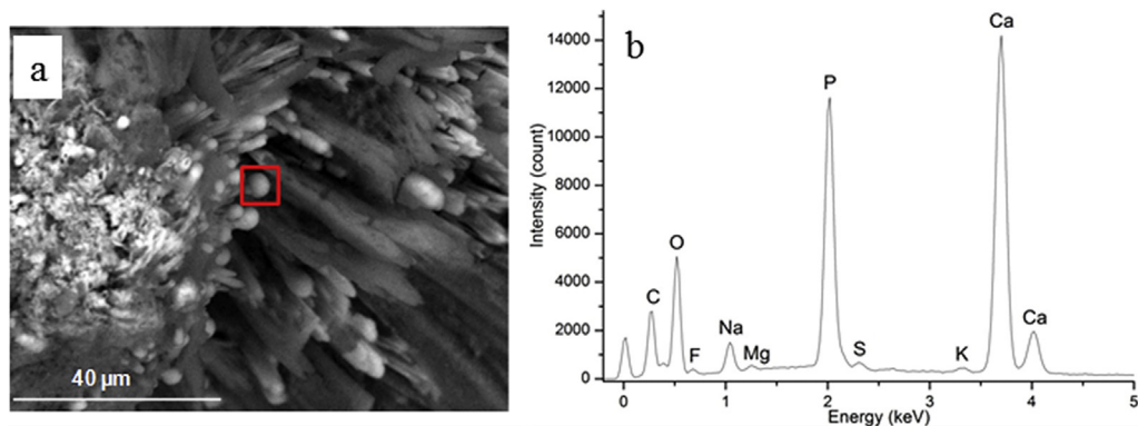
Fig. 3. (a) At the extremity of some NaUr needles, white spherical entities are visible (b) Elementary composition through EDS of the white spherical entities show that these entities are made of Ca, P and O.
