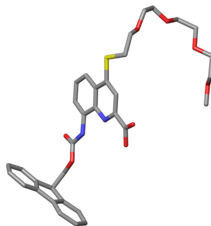
Fig. 2. Crystal structure of monomer 4. Hydrogen atoms have been omitted for clarity.
