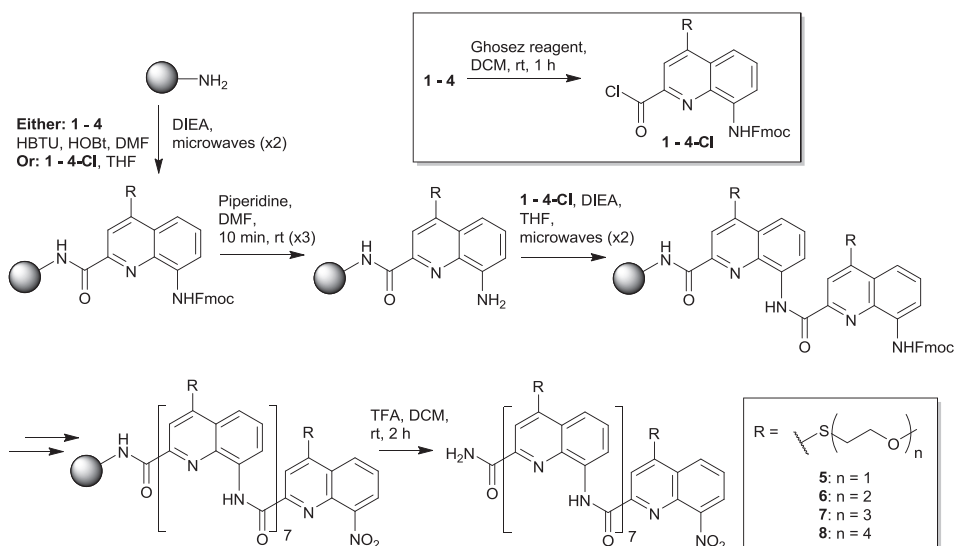
Scheme 2. SPS of OEG functionalized octamers.
