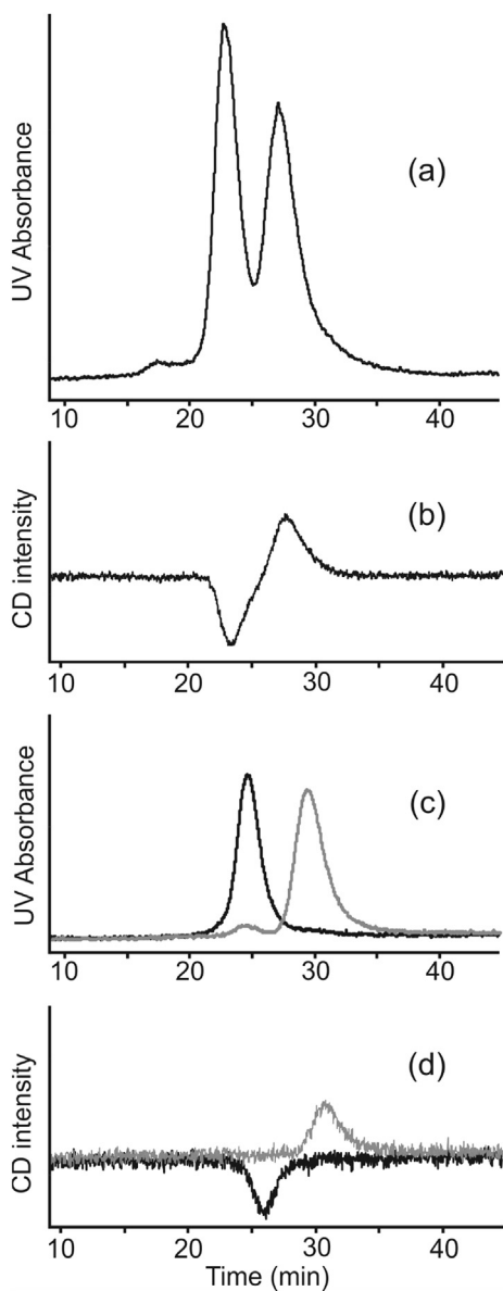
Fig. 3. Chiral HPLC separation of P and M helices of compound 8 at -5\text{ }^{\circ}\text{C} in MeOH/CHCl 3 (75:25). Expansion of: (a) UV detector trace (254 nm); (b) CD detector trace (385 nm). Overlaid expansions of isolated P - 8 (gray) and M - 8 (black); (c) UV detector traces (254 nm); (d) CD detector traces (385 nm).
