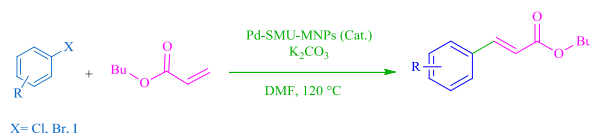
Scheme 3. Pd-SMU-MNPs catalyzed the Heck reaction.
