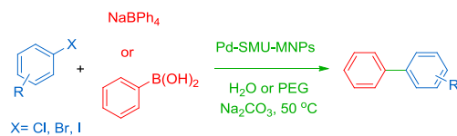
Scheme 2. Pd-SMU-MNPs catalyzed the Suzuki reaction.
