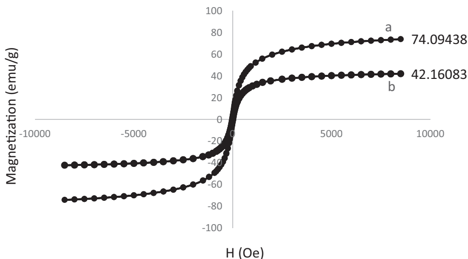
Fig. 5. Magnetization curves of \text{Fe}_3\text{O}_4 (a) and Pd-SMU-MNPs (b) at room temperature.
