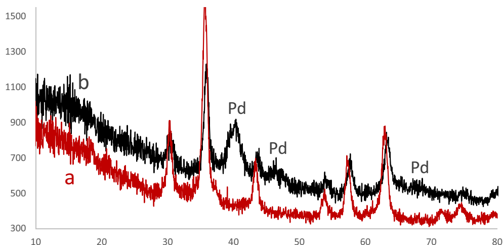
Fig. 3. XRD patterns of \text{Fe}_3\text{O}_4 nanoparticles (a) and Pd-SMU-MNPs (b).
