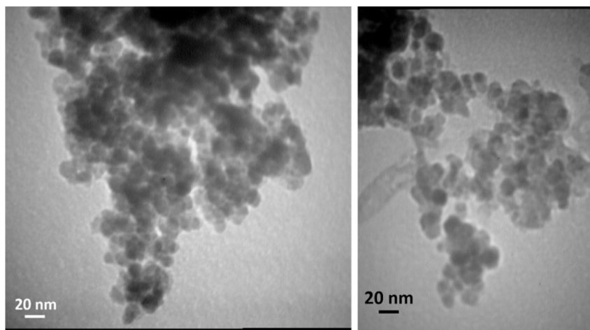
Fig. 2. TEM images of Pd-SMU-MNPs.
