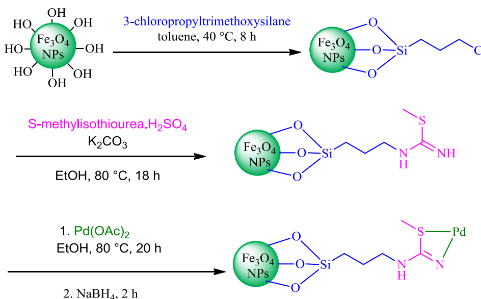
Scheme 1. Preparation process of Pd–SMU–MNPs.
