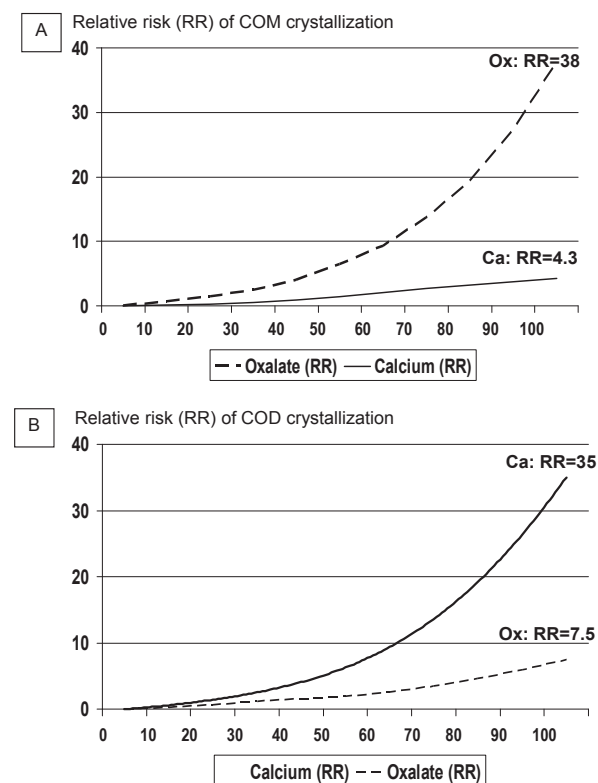
Fig. 5. Relative influence of calcium and oxalate concentration on the relative risk to form COM (Fig. 5A) and COD (Fig. 5B) crystals in the urine of stone formers.
