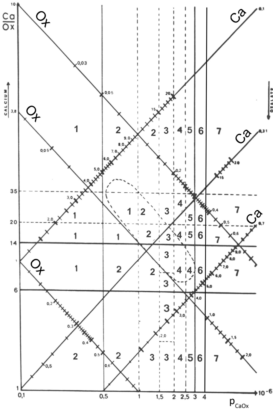
Fig. 7. Calcium oxalate crystallization nomogram with crystallization score values.
