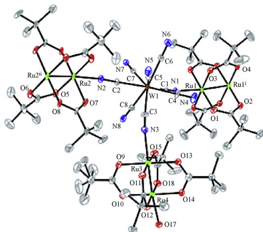
Fig. 3. ORTEP drawing of the molecular structure for \{[\text{Ru}^{\text{II}}\text{Ru}^{\text{III}}(\text{piv})_4(\text{H}_2\text{O})\{\text{W}^{\text{V}}(\text{CN})_8\}]\}^- moiety of 1 ·H 2 O, showing the thermal ellipsoids at the 50% probability level. Hydrogen atoms are omitted for clarity.
