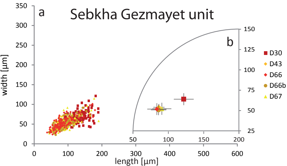
Supplementary figure 2: Overview of the morphological features length and width for all single grains (a) as well as the mean value for each sample (b), and roundness for the Sebkhya Gezmayet unit (c). The error bars in b, visualise the standard deviation for length and width within each sample.
