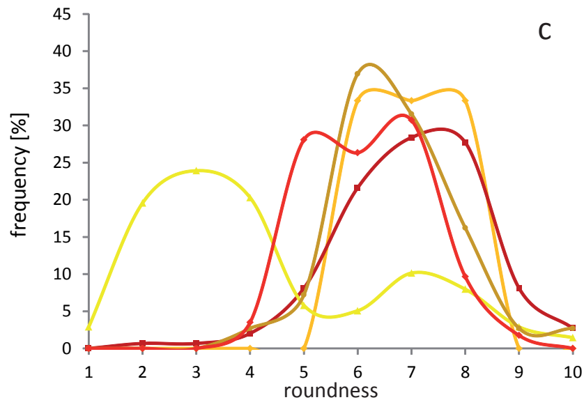
Supplementary figure 2: Overview of the morphological features length and width for all single grains (a) as well as the mean value for each sample (b), and roundness for the Sebkhya Gezmayet unit (c). The error bars in b, visualise the standard deviation for length and width within each sample.
