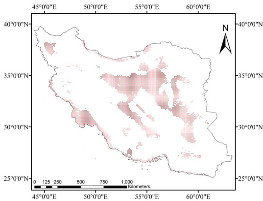
Figure 5. Detected points as saline soil in the study area based on procedure 1.
