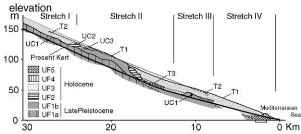
Fig. 3. Upstream-downstream distribution of lithological units. UF1 to UF5: alluvial units; UC1 to UC3: colluvial units; T1 to T3: alluvial terraces.
