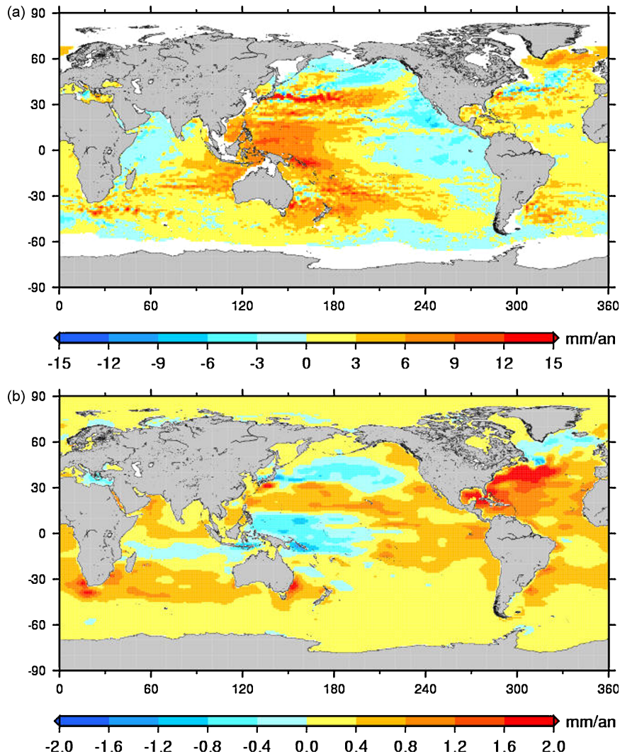
Fig. 4. a. Spatial patterns in thermal expansion trends over 1993–2003 (data from [15]). b. Spatial patterns in thermal expansion trends over 1955–2003 (data from [18]).
