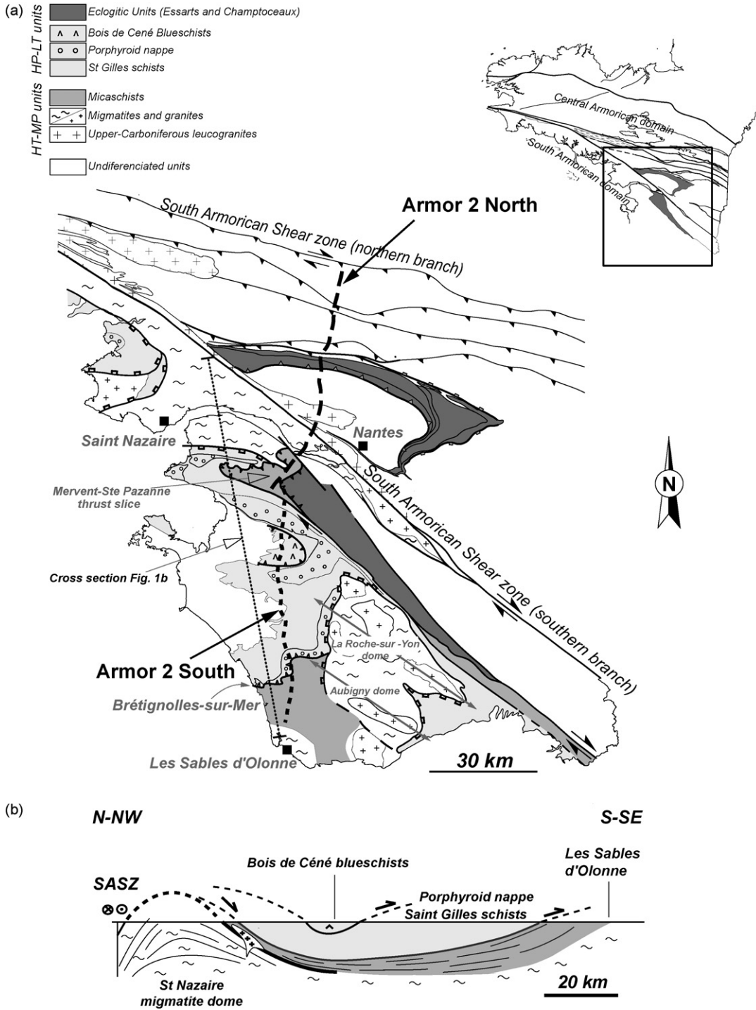
Fig. 1. a: location of the ARMOR 2 North and ARMOR 2 South seismic profiles on a simplified geological map; b: sketch cross-section (located on (a), modified after [Cagnard et al., 2004]).
