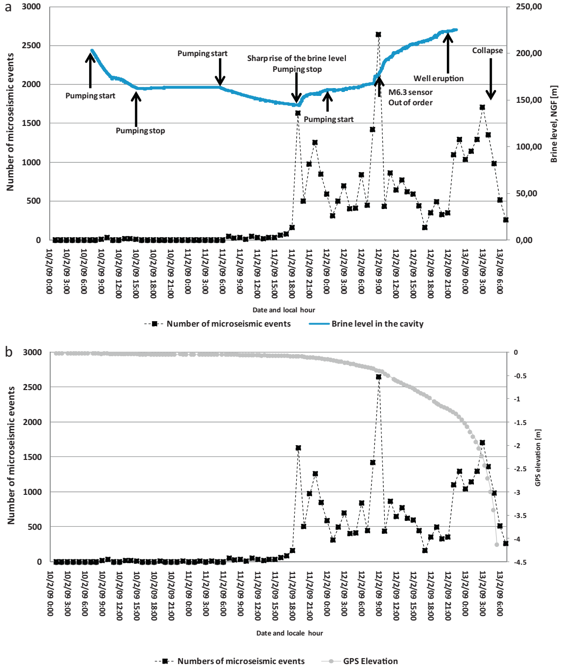
Fig. 3. a: number of microseismic events recorded on site and brine level measured at one extraction well (1 km distant from the cavern) between February 10 and 13, 2009. Note that microseismic peaks are correlated with rises in brine level; b: number of microseismic events recorded on site and subsidence measured by the GPS device. Note the strong acceleration in subsidence during the last 24 hours and the last GPS measurement indicating a cumulative subsidence of 4 m in the center of the area, before the ground collapse and flooding of the area.
