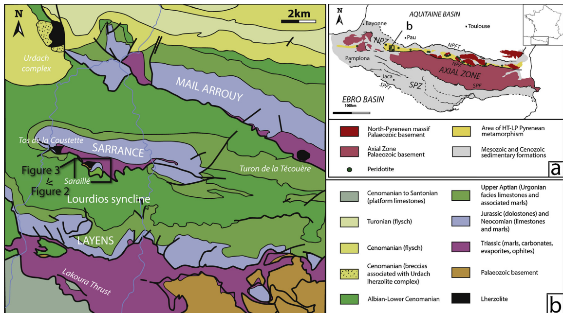
Fig. 1. a. Structural map of the Pyrenees. NPFT: North-Pyrenean Frontal Thrust, NPF: North-Pyrenean Fault, SPF: South-Pyrenean Fault, SPFT: South Pyrenean Frontal Thrust (after Vauchez et al., 2013). b. Structural map of the Chaînons Béarnais region, with location of the panoramic view of Fig. 2 and of map in Fig. 3 (rectangle) (after Castéras, 1970 and Lagabrielle et al., 2010).
