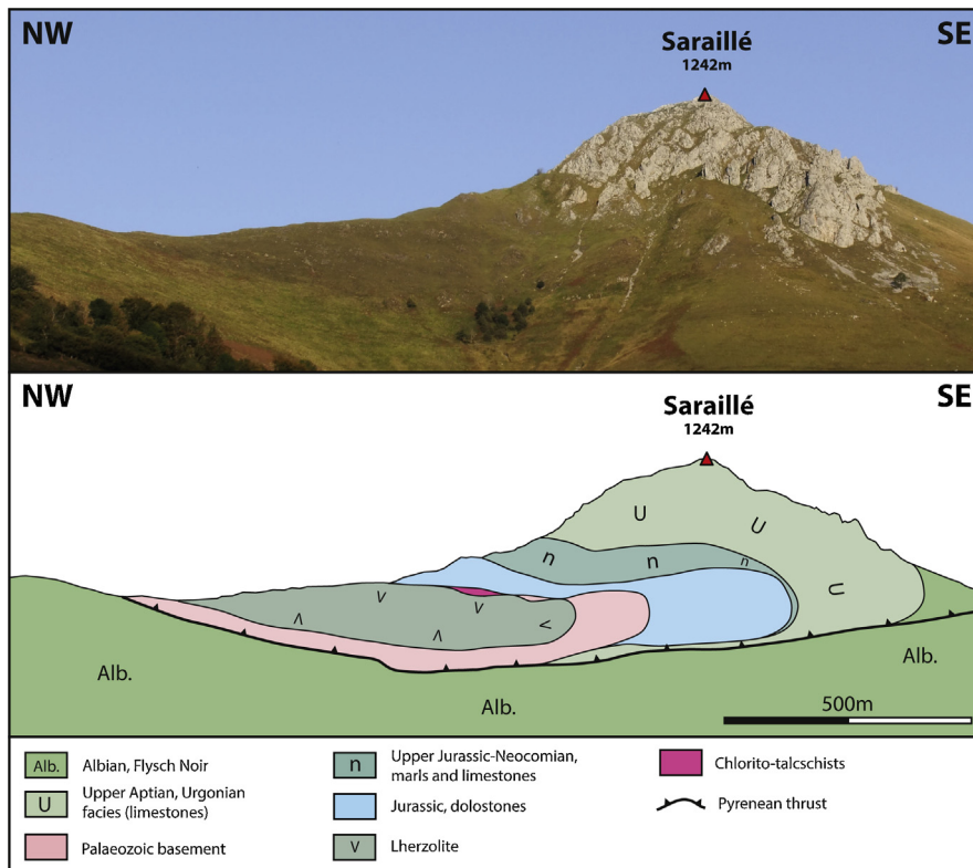
Fig. 2. Interpreted panorama of the Saraillé massif seen from the Lourdios syncline (see Fig. 1).
