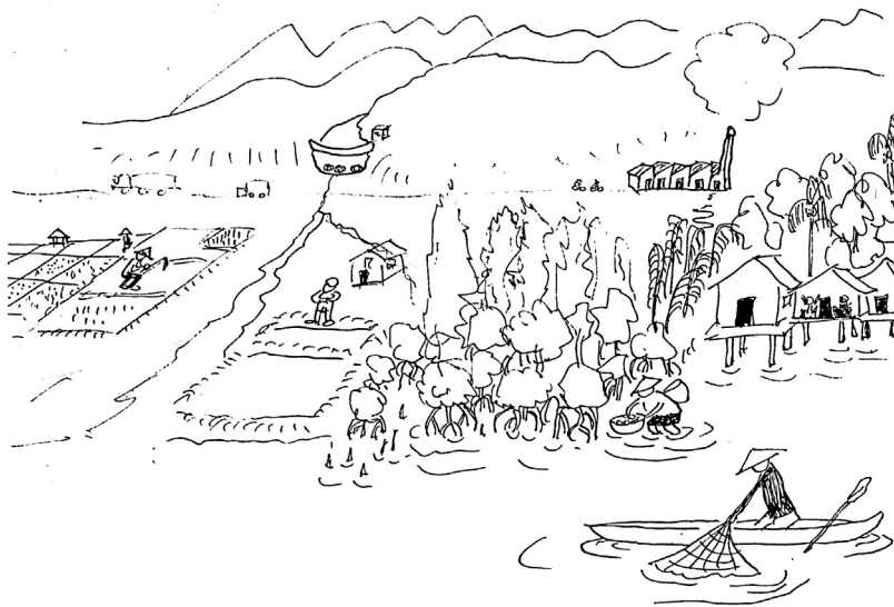
Fig. 2. Mangrove, a complex socio-ecosystem with multiple stakeholders, from local to global scales, which needs an interdisciplinary approach. Original drawing is courtesy of Dominique Guillaud, PALOC, Paris, December 2016.
