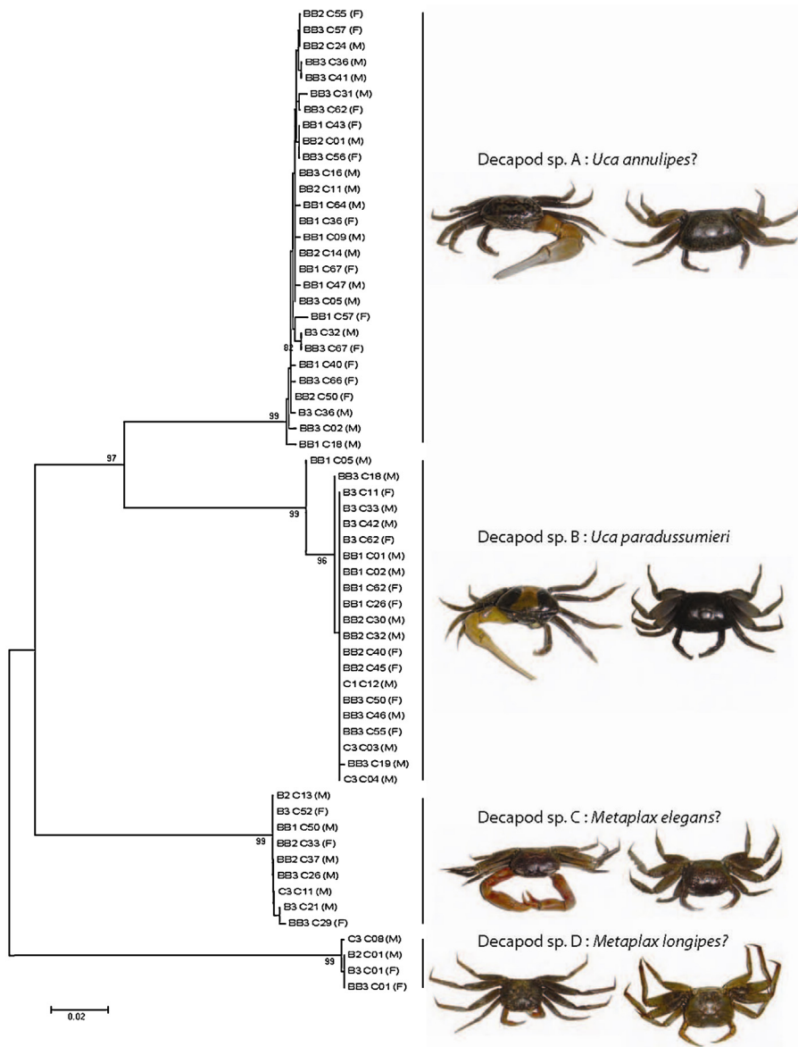
Fig. 5. Phylogenetic tree of the crabs sampled in the Can Gio Mangrove Biosphere Reserve in June 2015. Four species only were identified: Uca annulipes , U. paradussumieri , Metaplex elegans , and M. longipes .
