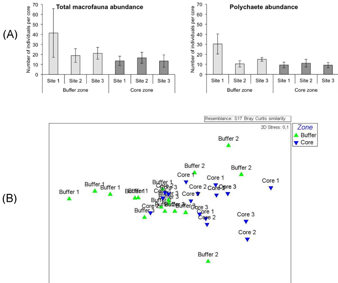
Fig. 4. A. Abundance (mean number of individuals \pm SE) of total macrofauna and polychaetes in the six replicates at the three sampling sites in the buffer and the core zones. B. Multidimensional scaling plot on the abundance data of each macrofauna group at the three sites (1–3) in the buffer zone (green triangles) and the core zone (blue inverted triangles). V = 6 .
