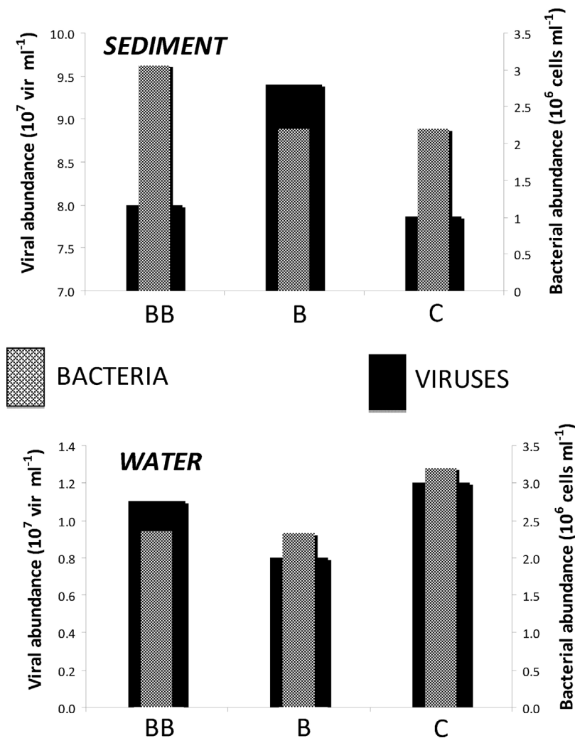
Fig. 3. Bacterial and viral abundance in the sediment and water in three zones in the Can Gio Mangrove Biosphere Reserve: buffer-bis zone (BB), buffer zone (B), and core zone (C).
