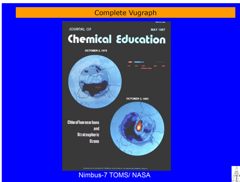
Fig. 2. Reproduction by the Journal of Chemical Education of another vugraph presented by Bhartia et al. (1985). It shows two images of Antarctic ozone taken on the same day (October 3) but four years apart. Large decrease of total ozone over Antarctica with no discernable change in lower latitudes seen in these images contradicted the model results predicting 1%/decade decrease in global total ozone due to CFCs. Comparison with Fig. 1 shows a rotating evolving Ozone Hole that expanded in just 2 days to reach the tip of South America.
