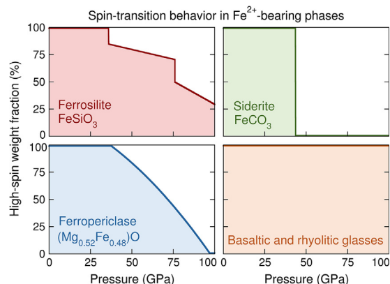
Fig. 9. High-spin ferrous iron weight fraction as a function of pressure up to 100 GPa at 300 K for four phases: single-crystal ferrosilite, \text{FeSiO}_3 (this study); single-crystal siderite, \text{FeCO}_3 (Lavina et al., 2009; Liu et al., 2015); powdered ferropicroclase, (\text{Mg}_{0.52}\text{Fe}_{0.48})\text{O} (Solomatova et al., 2016); and silicate glasses (Solomatova et al., 2017). In this study, we have determined that ferrosilite undergoes a two-stage spin transition: at about 37 and 76 GPa, the M1 and M2 sites begin to undergo a spin transition, respectively. The total high-spin weight fraction in ferrosilite drops from 100% to 85% at ~37 GPa and from 72% to 47% at ~76 GPa. At 100 GPa, about a third of the iron sites remain in the high-spin state. The step-wise spin-transition behavior in ferrosilite is unique in comparison to the other phases. Siderite undergoes a sharp spin transition at about 42 GPa, while ferropicroclase undergoes a gradual high-spin-to-low-spin transition, completing the spin transition by about 95 GPa. The silicate glasses do not undergo a spin transition up to at least 100 GPa. The weight fraction of high-spin atoms in ferropicroclase within the mixed-state region was fitted with a polynomial curve while for ferrosilite, the three segments (0–37 GPa, 37–76 GPa, and 37–100 GPa) were fitted linearly.
