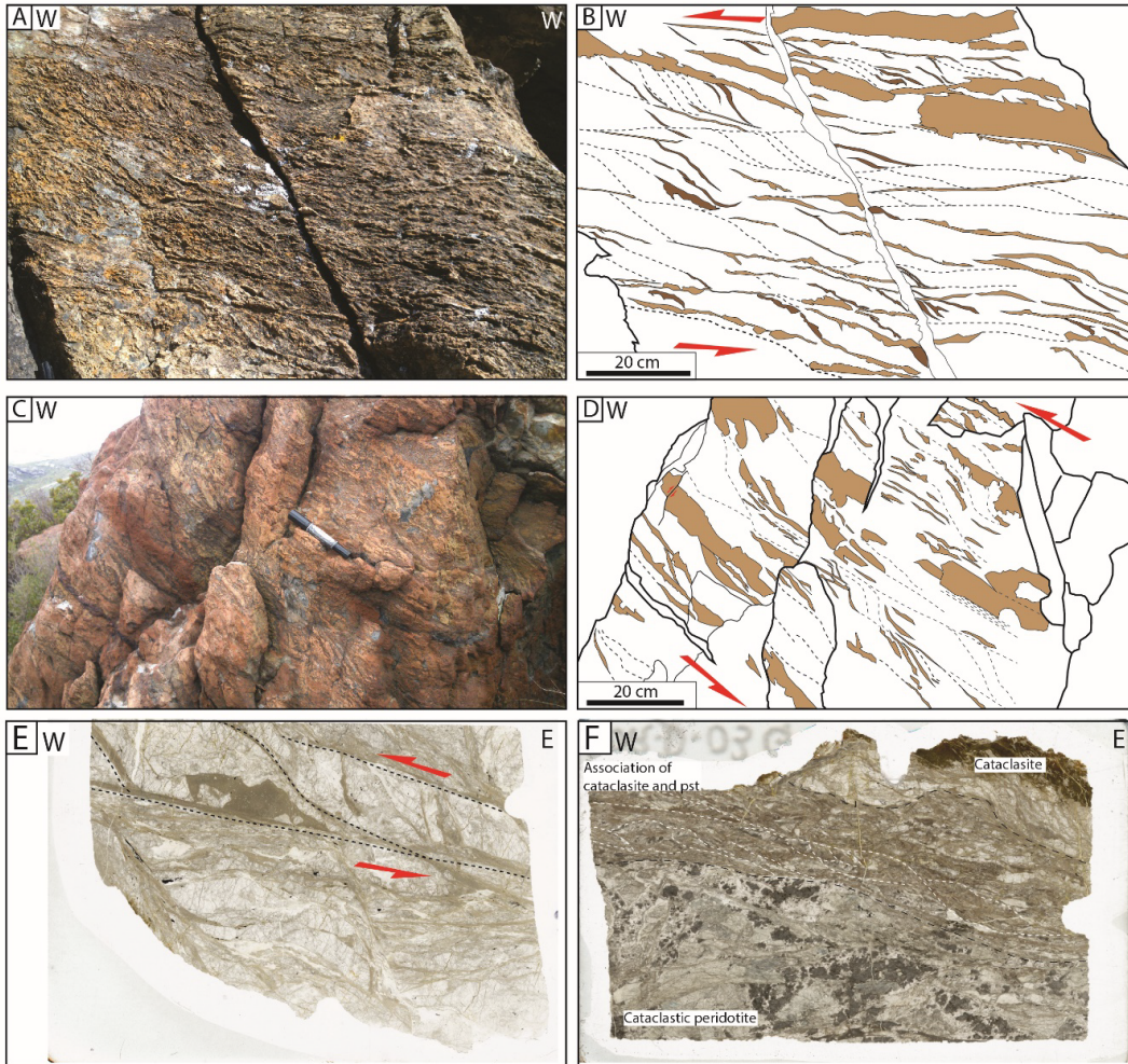
Figure 6. Pseudotachylyte and cataclasite in the Cima di Gratera ultramafic sub-unit. (A)–(B) Flat-lying pseudotachylyte veins (light brown) cross-cutting steeply dipping veins (dark brown) near \varphi_2 contact. (C)–(D) Steeply dipping pseudotachylyte veins associated to cataclasite bands (dark brown in (C)). (E) Thin section showing association of cataclastic bands with flat-lying pseudotachylyte. (F) Polyphase pseudotachylyte/cataclasite flat-lying shear band displaying S–C microstructure.
