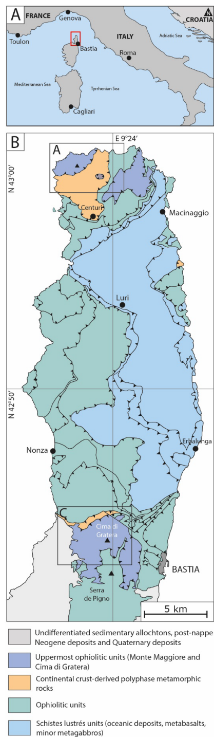
Figure 1. (A) Geographical setting of Corsica. (B) Geological setting of the studied ophiolitic units in Cape Corse. Insets (A) and (C) refer to maps (A) and (C) of Figure 2.
