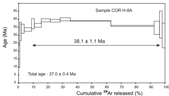
Figure 4. ^{40}\text{Ar}/^{39}\text{Ar} age spectrum of the gabbro-hosted pseudotachylite injection vein COR H-8A. The double arrow indicates the range of released cumulative ^{39}\text{Ar} (%) regarded as a plateau from which the 38.1 Ma age of formation is derived.
