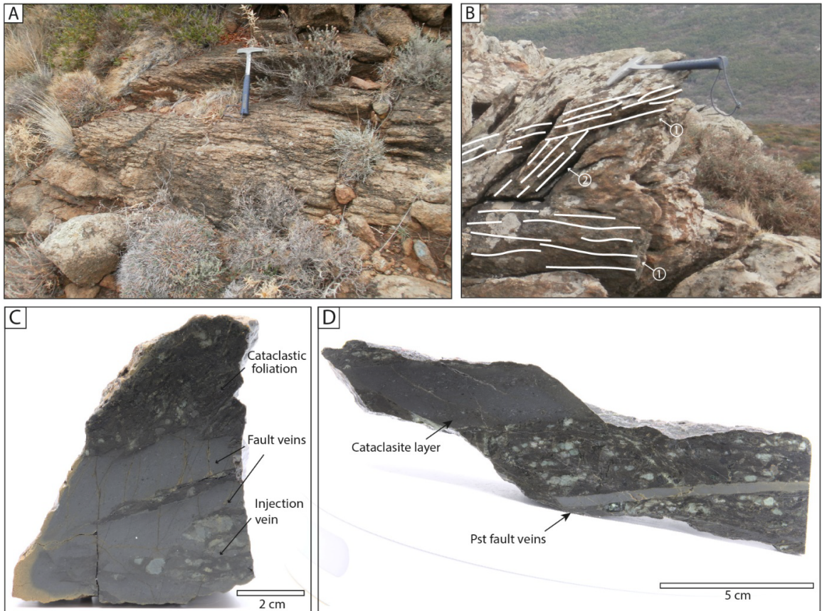
Figure 3. Cataclastic foliation and pseudotachylite and cataclasite veins in the Monte Maggiore ultramafics. (A) Flat-lying cataclastic foliation. (B) Gently dipping cataclastic foliation (2) deflected by a flat-lying cataclastic foliation (1). (C) Serpentinized peridotite hand-sample- hosting flat-lying pseudotachylite veins. (D) Foliated serpentinite hand-sample showing a flat-lying pseudotachylite vein and a cataclastic layer.
