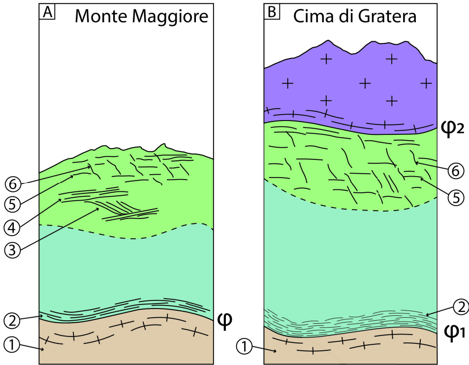
Figure 7. Summary of the geometry of pseudotachylyte veins, cataclastic layers and cataclastic foliation in the Monte Maggiore and Cima di Gratera units. Keys to numbers: (1) Foliated paragneiss or orthogneiss of the continental crust-derived basal units. (2) Foliated serpentinite along the basal thrust surfaces. (3) Steeply dipping cataclastic foliation. (4) Flat-lying cataclastic foliation. (5) Flat-lying pseudotachylyte fault veins and cataclastic zones. (6) Steeply dipping pseudotachylyte fault veins and cataclastic zones.
