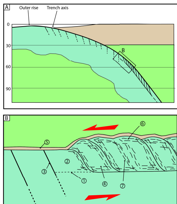
Figure 8. Interpretative model for underplating of the uppermost part of the subducting Piemonte-Ligurian oceanic lithosphere. (A) General framework showing outer rise bending-related normal faulting near the trench, and propagation and underplating at depth. (B) Enlarged view of the forward propagation of the thrust sheets through imbrication. Keys to numbers: (1) Propagating basal thrust surface. (2) Soon-to-be incorporated thrust sheet. (3) Outer-rise normal fault prone to reactivation as a thrust sheet-bounding fault. (4) Underplated thrust sheet. (5) Metamorphosed basalts and sedimentary cover. (6) Flat-lying structures (pseudotachylyte fault veins, cataclastic veins, cataclastic foliation). (7) Steeply dipping structures (pseudotachylyte fault veins, cataclastic layers, cataclastic foliation).
