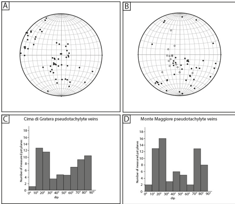
Figure 5. Attitude of pseudotachylyte veins, cataclastic layers and cataclastic foliation in ultramafic rocks. (A) Lower hemisphere equal-area projection of poles to pseudotachylyte fault veins in the Cima di Gratera ultramafic sub-unit (56 measurements). (B) Lower hemisphere equal-area projection of poles to pseudotachylyte fault veins (solid circles), cataclastic layers (triangles) and cataclastic foliation (open circles) surfaces in the Monte Maggiore ultramafic rocks (61 measurements). (C) Histogram showing the distribution of dip angles for pseudotachylyte fault veins at Cima di Gratera. (D) Same for Monte Maggiore.
