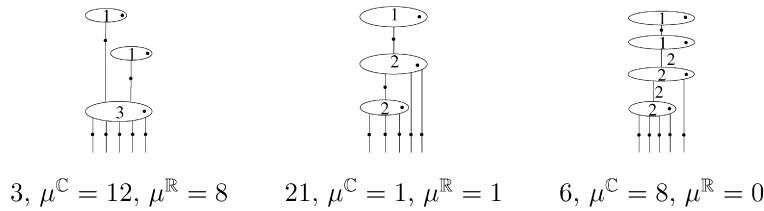
Fig. 2. 3-dimensional marked floor diagrams of degree 5, genus 0, and marked by 10 points.
