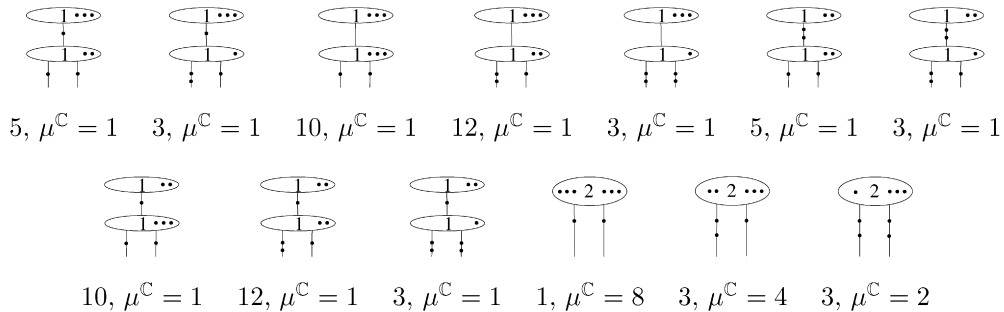
Fig. 3. 3-dimensional marked floor diagrams of degree 2, genus 0, and marked by 8 lines.
