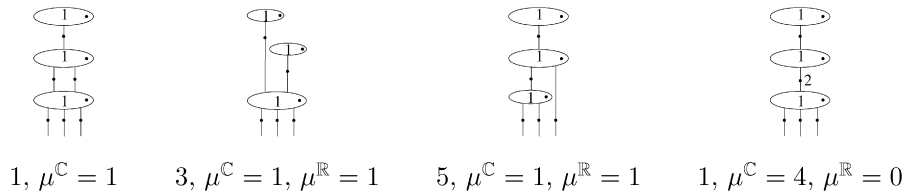
Fig. 1. 2-dimensional marked floor diagrams of degree 3.
