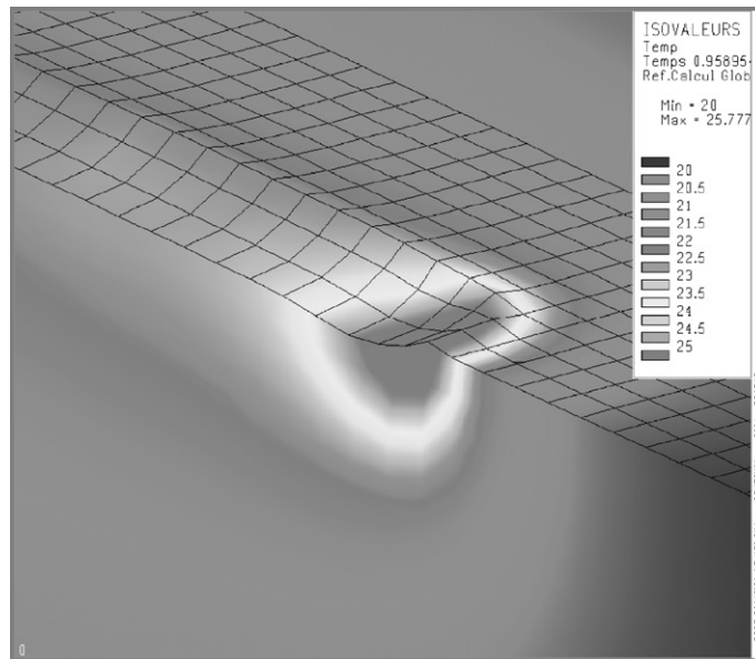
Temperature field in a glassy polymer during scratching
