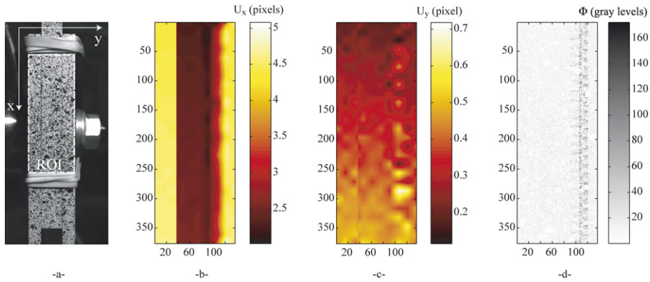
Fig. 2. (a) Analyzed bolted assembly and rectangular region of interest (ROI) delimited by a white dashed line. (b) Vertical displacement field in pixels. (c) Horizontal displacement field. (d) Gray level residual map.
