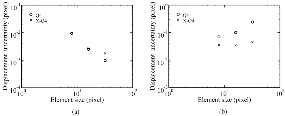
Fig. 3. Displacement uncertainties as a function of element size for a Q4 and an extended (X-Q4) algorithm when a uniform displacement is prescribed (a), and a discontinuous displacement (b).
