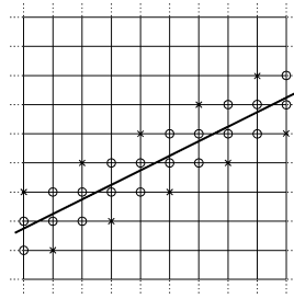
Fig. 1. Discontinuous enrichment on a typical mesh. Circles denote nodes that hold discontinuous degrees of freedom, cross nodes that hold discontinuous degrees of freedom considered as fixed.
