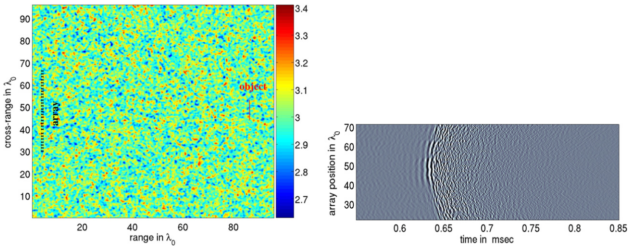
Fig. 3. Array imaging in clutter. The computational set-up is shown on the left. The fluctuations in the sound speed are shown in color and the color-bar is in km/s. The traces received when illuminating from the central element in the array are on the right.
