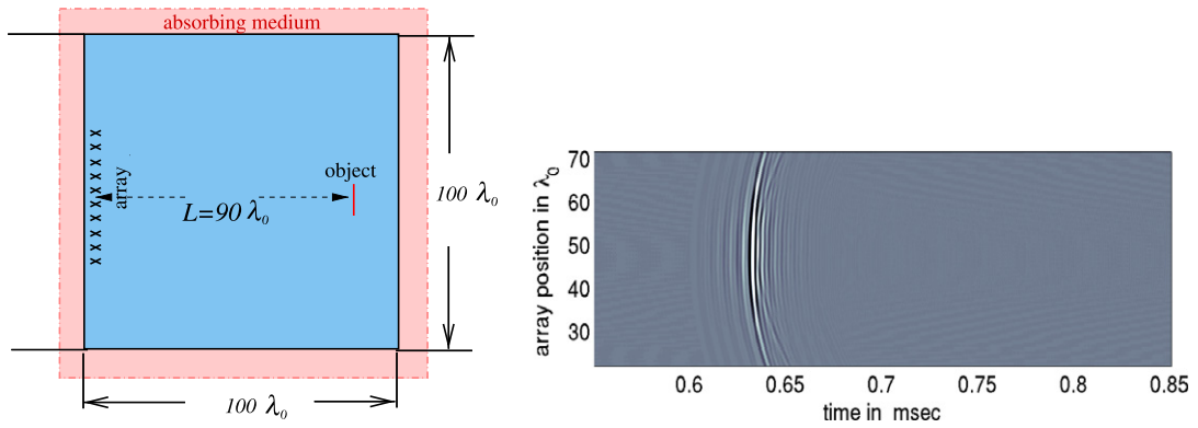
Fig. 2. Schematic of array imaging in a homogeneous medium. The computational set-up is on the left. The traces received when illuminating from the central element in the array are on the right.
