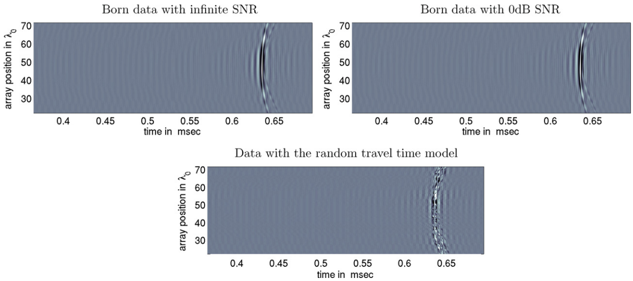
Fig. 4. Traces on the array for the central source illumination. Top: the response matrix is simulated using the linearized Born model. Bottom: the random travel time model is used to simulate the response matrix.
