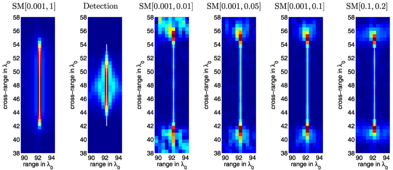
Fig. 10. Subspace migration results for the Born data with 0 dB SNR.
