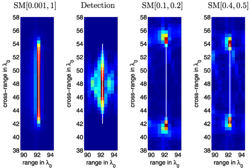
Fig. 11. Subspace migration results for the data obtained by solving the full wave equation in a homogeneous medium.
