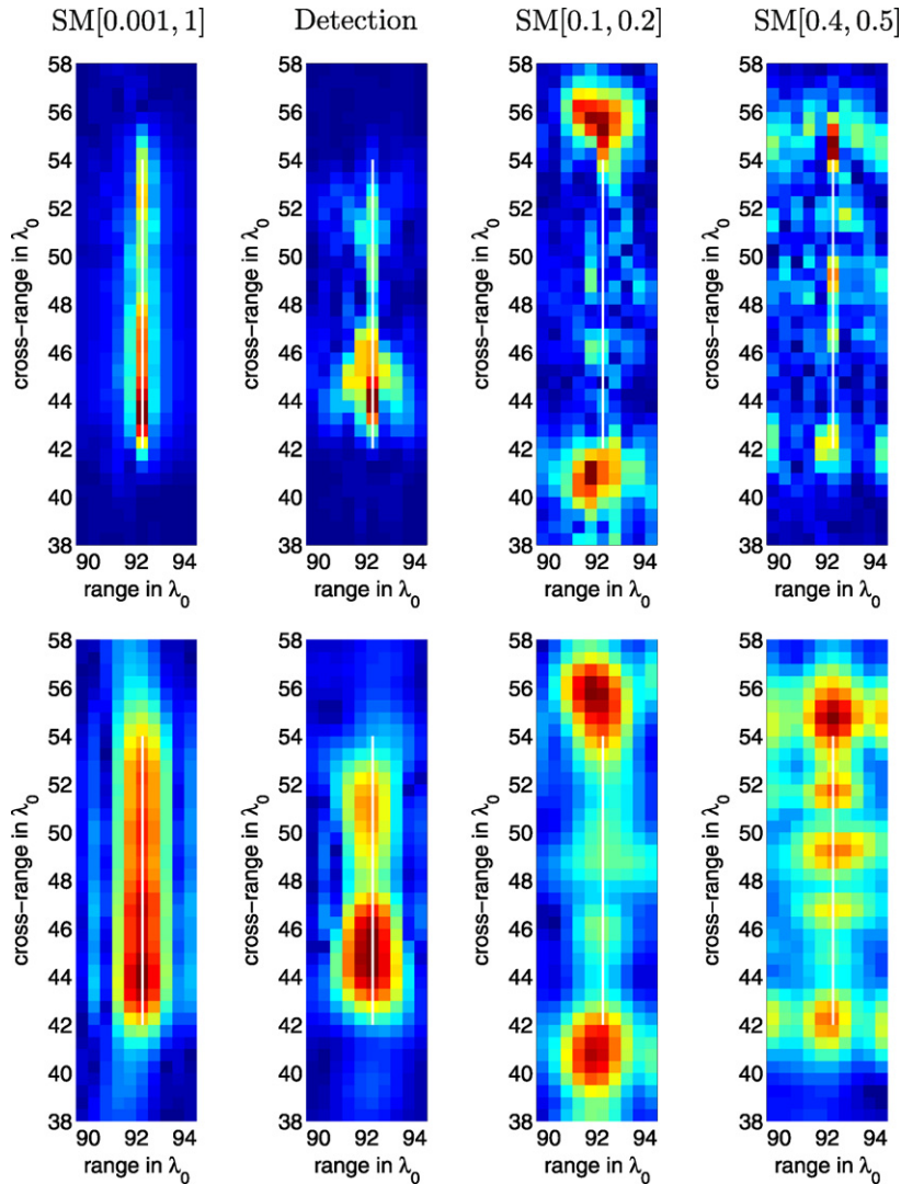
Fig. 12. Imaging results for the data obtained with the random travel time model. Top line: the imaging method used is migration. Bottom line: the imaging method used is coherent interferometry.
