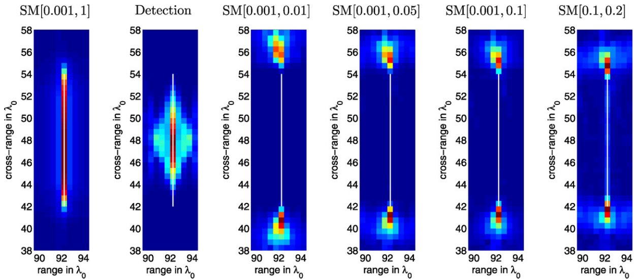
Fig. 9. Subspace migration results for the Born data with infinite SNR.
