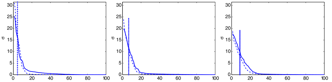
Fig. 7. The singular values of \widehat{\Pi}(\omega) for the cluttered medium (—) and the random travel time model (---) for frequencies 200 kHz (left), 300 kHz (middle) and 400 kHz (right). The vertical line in the figures is the theoretical transition value N(\omega) = \lfloor b/(\lambda L/a) \rfloor which is 5, 7 and 9, respectively.
