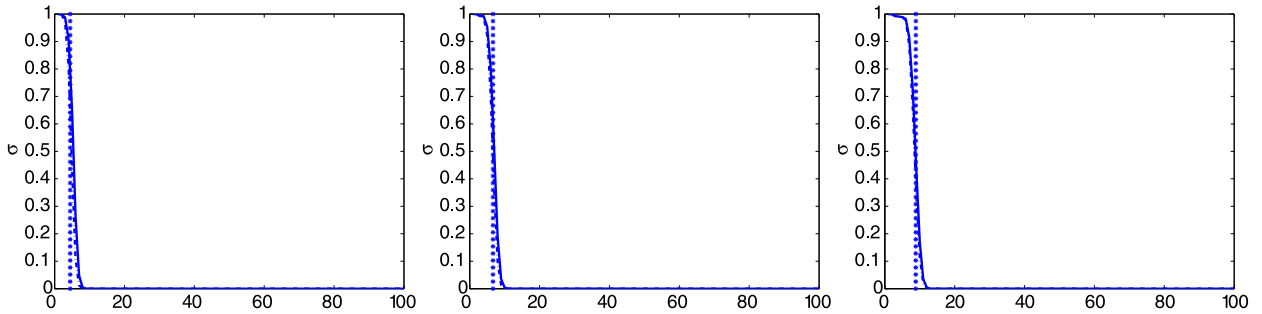
Fig. 5. The normalized singular values of \widehat{\Pi}(\omega) for the full wave data (—) and the Born data (---) for frequencies 200 kHz (left), 300 kHz (middle) and 400 kHz (right). The vertical line is the theoretical transition value N(\omega) = b/(\lambda L/a) which is approximately 5, 7 and 9 respectively.
