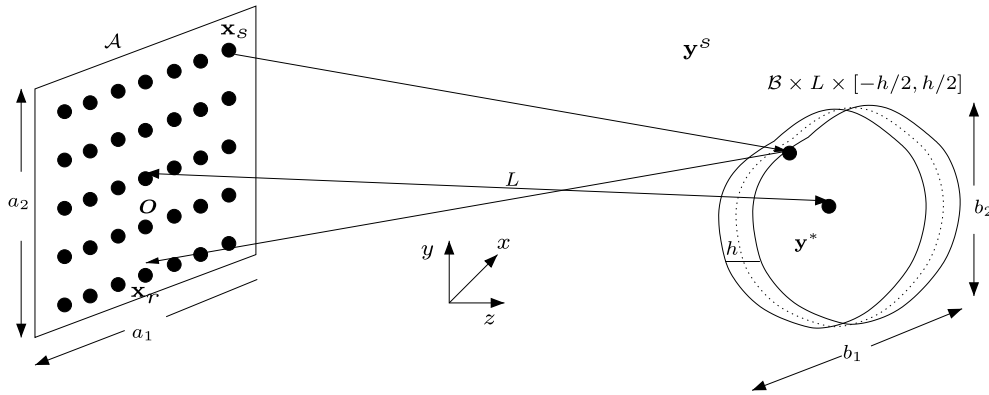
Fig. 1. Schematic for array imaging an extended reflector.
