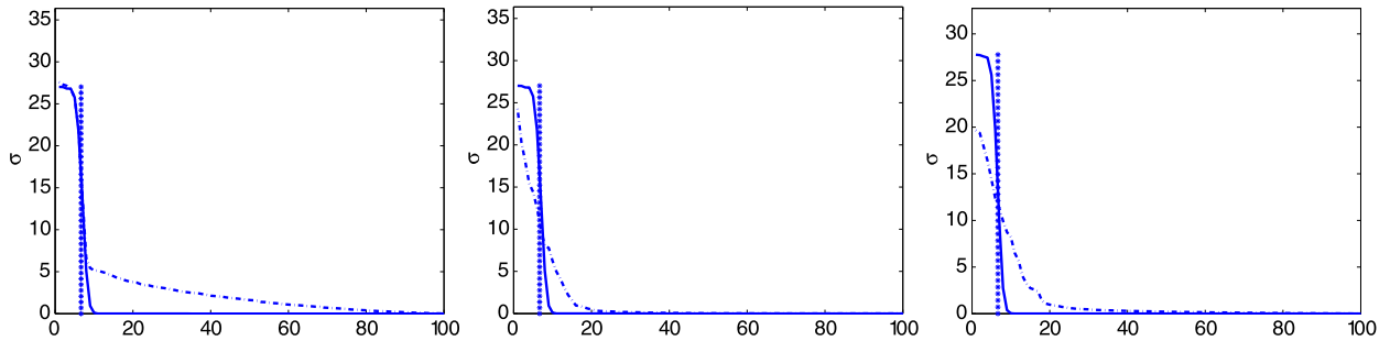
Fig. 6. The singular values of \widehat{\Pi}(\omega) at frequency 300 kHz. Left: the — line is for the Born data with infinite SNR and the ---- line is for the data with 0 dB SNR. Middle: the — line is for the Born data with infinite SNR and the ---- line is for the data obtained with the random travel time model. Right: the — line is for the homogeneous medium and the ---- line for the cluttered medium. The vertical line is the theoretical transition value N(\omega) = \lfloor b/(\lambda L/a) \rfloor which is 7.
