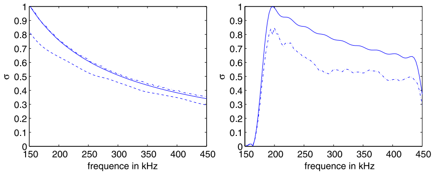
Fig. 8. The largest singular values of the response matrix \widehat{\Pi}(\omega) as a function of frequency. Left: the — line is for the Born data with infinite SNR, the --- line is for the data with 0 dB SNR and the -- line is for the data obtained with the random travel time model. Right: the — line is for the homogeneous medium and the --- line for the cluttered medium.
