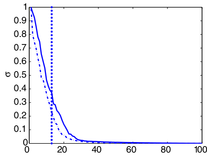
Fig. 14. The normalized singular values of \hat{\Pi}(\omega) for the cluttered medium (—) and the random travel time model (---) for the frequency of 400 kHz. The vertical line corresponds to the 13-th normalized singular value.
