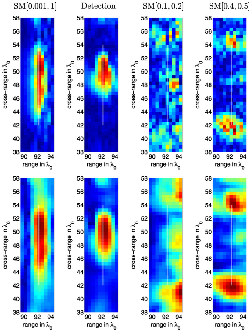
Fig. 13. Imaging results for the data obtained by solving the full wave equation in the cluttered medium shown in the left panel of Fig. 2. Top line: the imaging method used is migration. Bottom line: the imaging method used is coherent interferometry.
