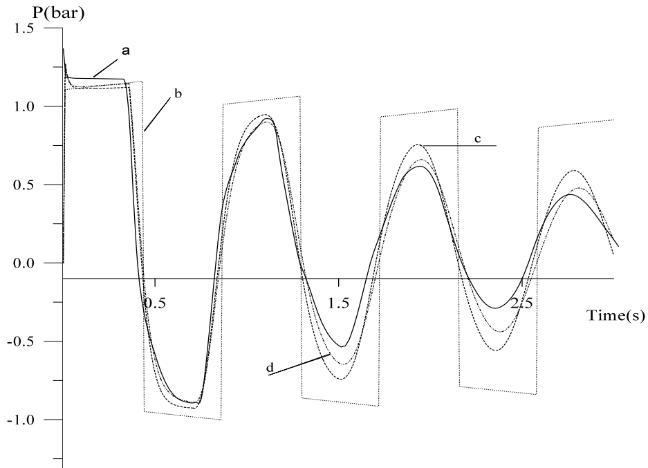
Fig. 3. Response of pressure at downstream end of polyethylene pipe on sudden closure of valve in classical model – comparison of theory and experiment at 25 °C.
