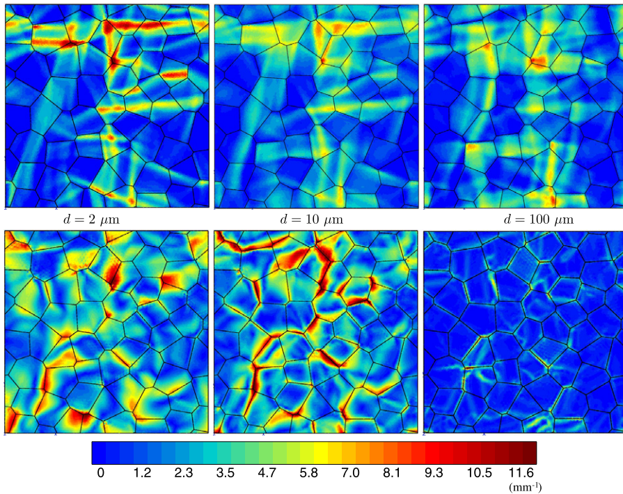
Fig. 7. Grain size effect on the accumulated plastic strain p (top figures) and on the norm of the dislocation density tensor \|\mathbf{L}\| (bottom figures). These contour plots are obtained with the 55-grain aggregate for the same mean value of \langle\chi_{12}^{ps}\rangle = 0.01 , and from the set of material parameters given in Table 2. The colour scale for the plastic strain field of the top figures is the same as that of Fig. 6 on the right. The colour scale at the bottom is that for the dislocation density tensor fields.
