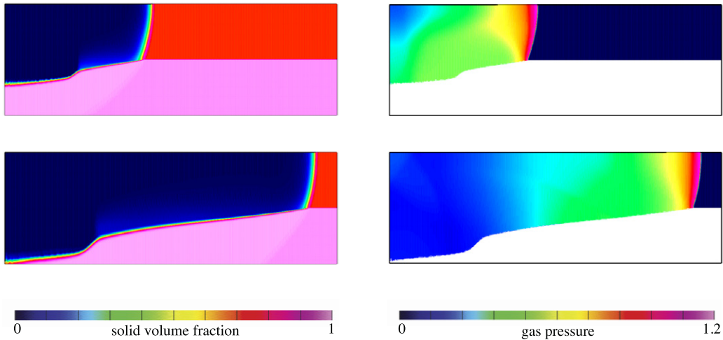
Fig. 3. Strong confinement: shaded contour plots of solid volume fraction and gas pressure for t = 1.5 (top) and t = 4.0 (bottom).
