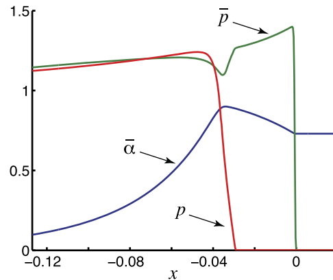
Fig. 2. Steady, one-dimensional structure of the rigidly-confined detonation.
