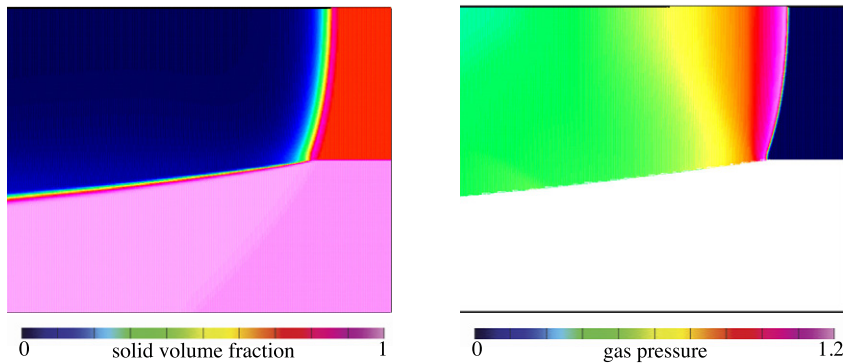
Fig. 5. Expanded views of the wavefront of the strongly-confined detonation at t = 4.0 : shaded contour plots of solid volume fraction (left) and gas pressure (right).
