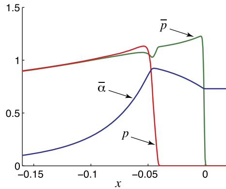
Fig. 4. Structure of the strongly-confined detonation at the symmetry plane.
