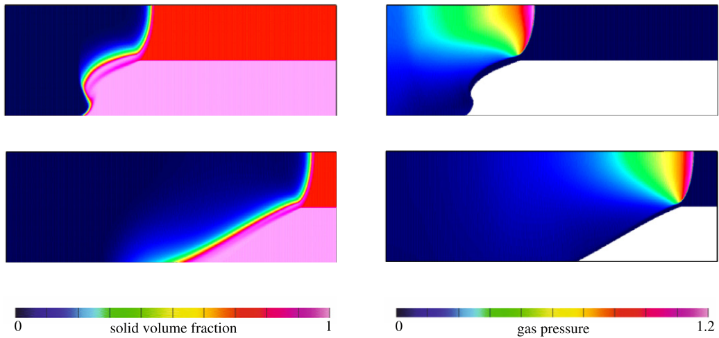
Fig. 6. Weak confinement: shaded contour plots of solid volume fraction and gas pressure for t = 1.5 (top) and t = 4.0 (bottom).
