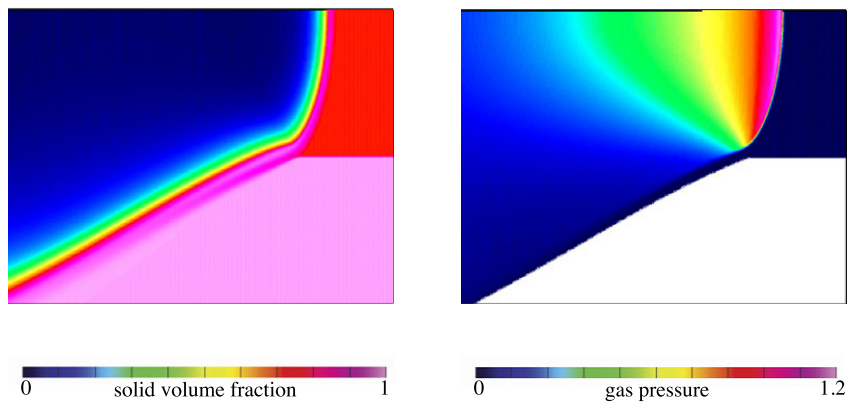
Fig. 8. Expanded views of the wavefront of the weakly-confined detonation: shaded contour plots of solid volume fraction (left) and gas pressure (right).
