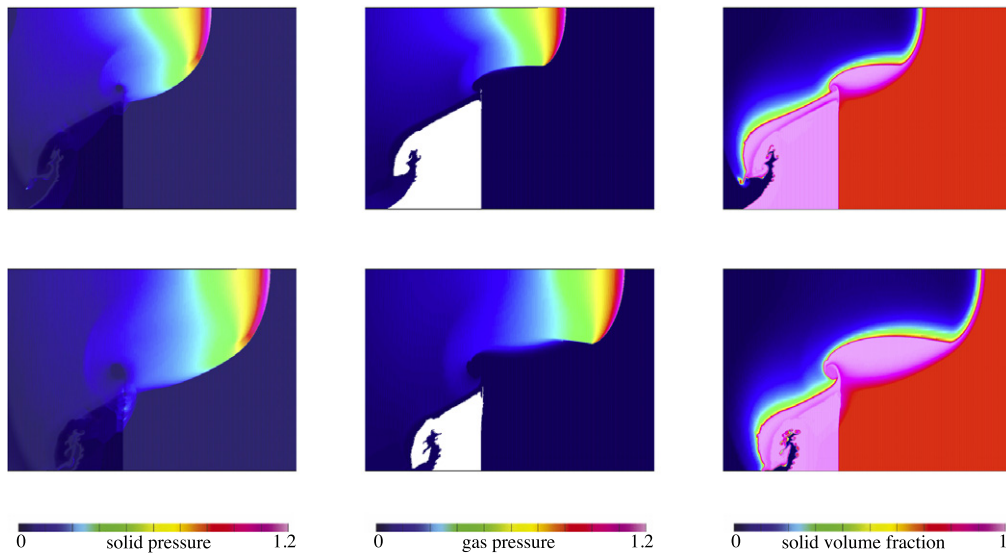
Fig. 14. Weak confinement: solid pressure (left), gas pressure (middle) and solid volume fraction (right) at t = 4.0 (top frames) and t = 5.0 (bottom frames).
