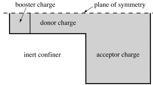
Fig. 1. Initial configuration for corner turning. A detonation in the donor segment, initiated by the booster, will propagate to the right and diffract into the acceptor segment.
