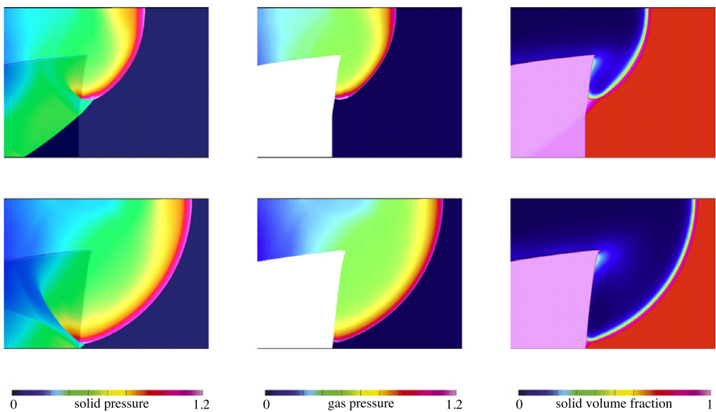
Fig. 11. Strong confinement: solid pressure (left), gas pressure (middle) and solid volume fraction (right) at t = 4.0 (top frames) and t = 5.0 (bottom frames).
