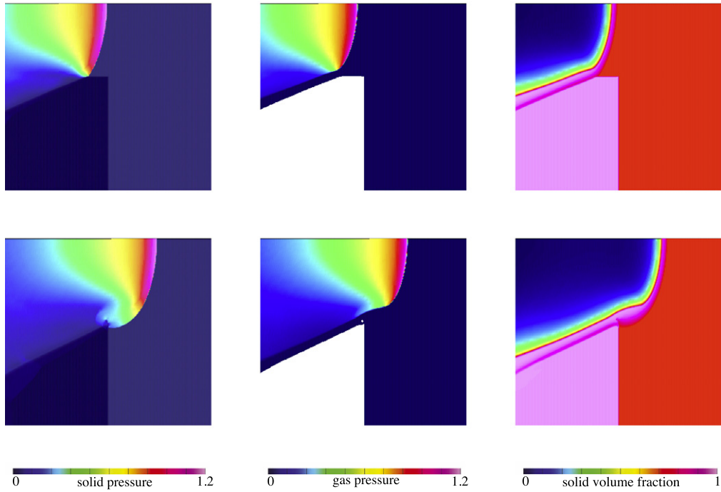
Fig. 12. Weak confinement: solid pressure (left), gas pressure (middle) and solid volume fraction (right) at t = 2.6 (top frames) and t = 3.2 (bottom frames).
