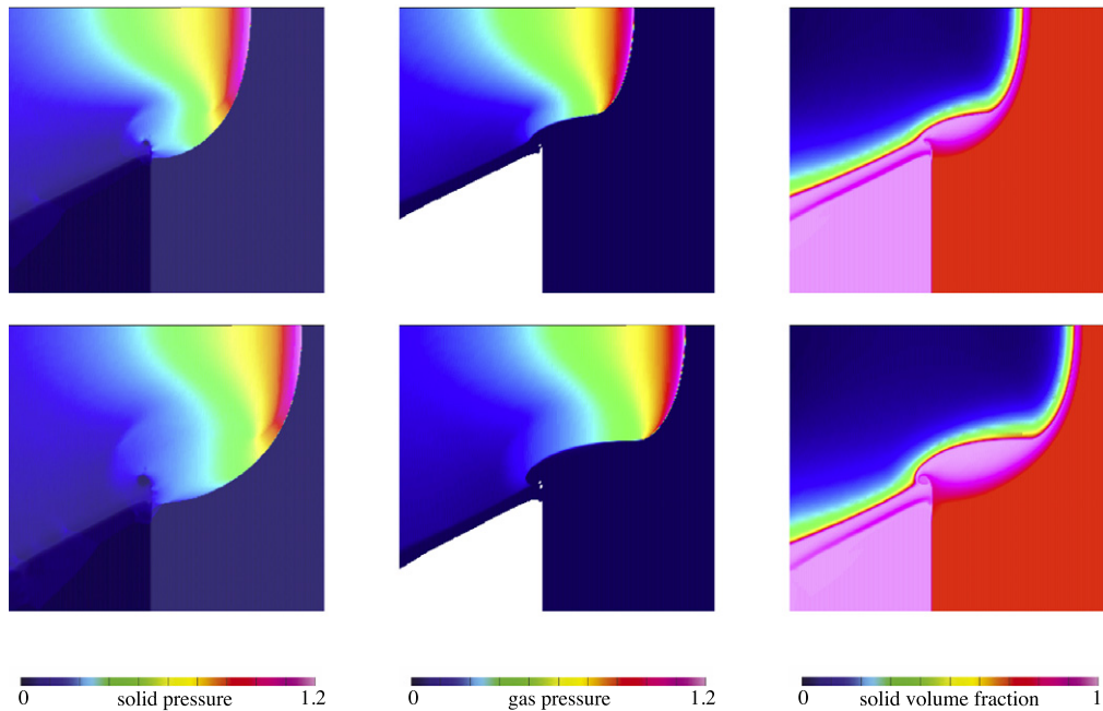
Fig. 13. Weak confinement: solid pressure (left), gas pressure (middle) and solid volume fraction (right) at t = 3.4 (top frames) and t = 3.8 (bottom frames).
