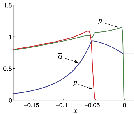
Fig. 7. Structure of the weakly-confined detonation at the symmetry plane.
