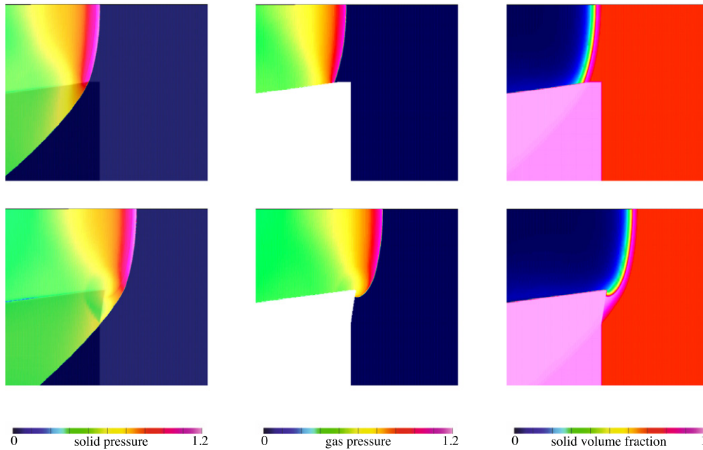
Fig. 9. Strong confinement: solid pressure (left), gas pressure (middle) and solid volume fraction (right) at t = 2.6 (top frames) and t = 3.0 (bottom frames).
