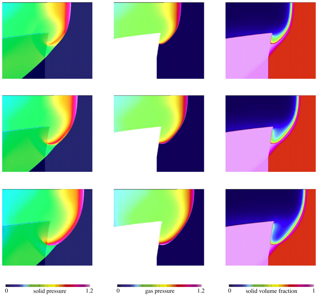
Fig. 10. Strong confinement: solid pressure (left), gas pressure (middle) and solid volume fraction (right) at t = 3.4 (top frames), t = 3.6 (middle frames) and t = 3.8 (bottom frames).
