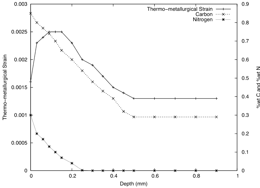
Fig. 13. Carbonitrided specimen: in-depth thermo-metallurgical strain profile (component xx ) depending on the percentage of carbon and nitrogen at 25 °C (results obtained using JMatPro).
