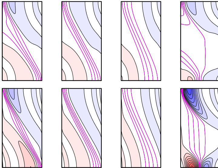
Fig. 5. Contours of the angular velocity \omega = v/r , for Ha^2 = 10^6 , and with B_\phi = 10r^{-1}\hat{\mathbf{e}}_\phi added to the previous choices Fields 1–4. All eight panels are exactly as in Fig. 2, except that the contour interval is now 0.2 throughout, for both the magenta and the black contour lines. (Color online.)
