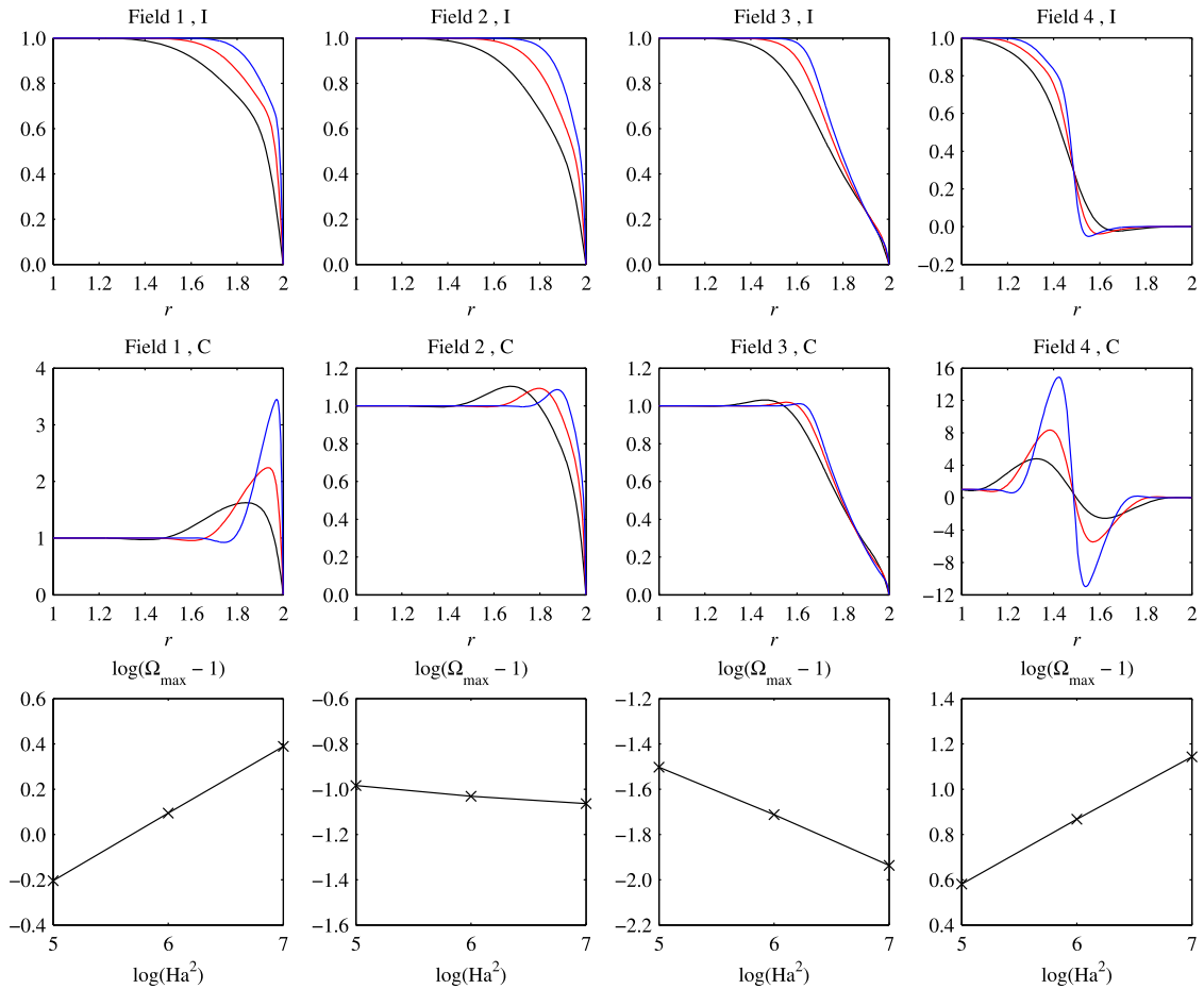
Fig. 3. The first two rows show \omega(r) at z=2 , for Fields 1–4 from left to right as indicated, the first row insulating (I) and the second row conducting (C). Within each panel black–red–blue indicate Ha^2 = 10^5, 10^6, 10^7 , respectively. The third row shows how the amplitude of the super-rotation in the second row scales with Ha , and suggests fits of the form Ha^s , with s \approx 0.59, -0.08, -0.43, 0.56 , respectively. (Color online.)
