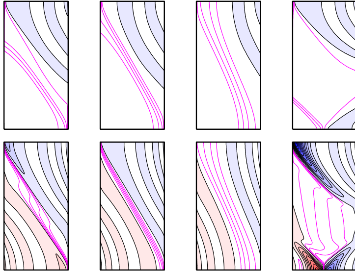
Fig. 2. Contours of the angular velocity \omega = v/r , for Ha^2 = 10^6 . From left to right are the four choices Fields 1–4. The top row is for insulating boundaries, the bottom row conducting. In each panel, only the upper half of the domain is shown; that is, r extends over the full range [1, 2] , but z \in [2, 4] . The lower half z \in [0, 2] is reflection-symmetric in each case, as seen also in Fig. 1. The white regions indicate values between 0 at the outer boundary and 1 at the inner; the magenta contour lines in these regions have intervals 0.2. The red-shaded regions correspond to super-rotation, where \omega > 1 ; the blue-shaded regions correspond to counter-rotation, where \omega < 0 . In both cases, the black contour lines in these regions have intervals 1. (Color online.)
