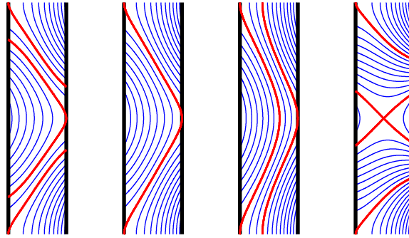
Fig. 1. From left to right, the four combinations that are referred to as Fields 1–4 in the text. The thick red lines in each case denote the special field lines across which the linkage to the boundaries changes, and where Shercliff layers are thus expected to arise. The general form is (\hat{\mathbf{e}}_z + c_I \mathbf{B}_I + c_K \mathbf{B}_K)/c_0 , where c_I and c_K are adjusted to select the desired field topology, and c_0 is then chosen to rescale the maximum amplitude to 1. The precise values of (c_I, c_K) are (0.155, -4.356) , (0.124, -3.485) , (0.091, -2.562) , (0.548, -7.687) , respectively. (Color online.)
