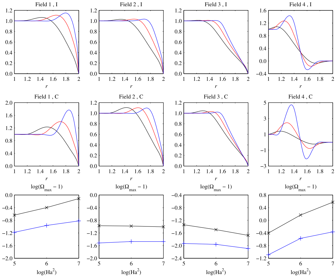
Fig. 6. As in Fig. 3, the first two rows show \omega(r) at z=2 , for Fields 1–4 and I and C as indicated. Within each panel, black, red, blue again corresponds to Ha^2 = 10^5, 10^6, 10^7 . In the third row, the blue lines (+ symbols) and the black lines (× symbols) show the scalings with Ha of the I and C super-rotations, respectively. (Color online.)
