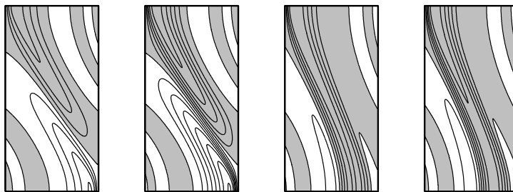
Fig. 7. Contours of \psi r , which constitutes the streamfunction of the meridional circulation \nabla \times (\psi \hat{e}_\phi) . From left to right Field 1, I and C boundaries, then Field 3, I and C boundaries, and Ha^2 = 10^6 for all four. White indicates negative values, grey positive. The contour intervals are 5 \cdot 10^{-3} for Field 1, and 10^{-3} for Field 3.
