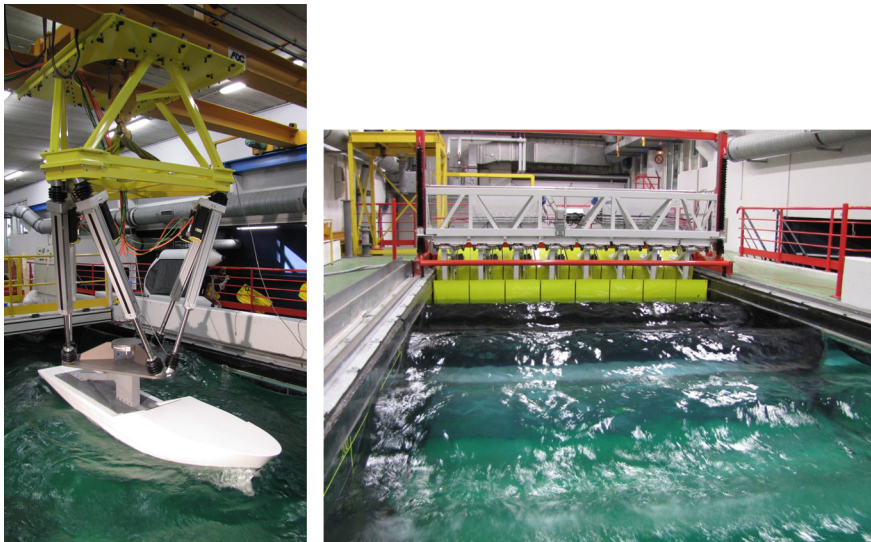
Fig. 2. Presentation of the 1/30 ship model with the ship motion generator system (left) and the wave generator system (right) generating regular waves with a current of 0.75 \text{ m s}^{-1} .
