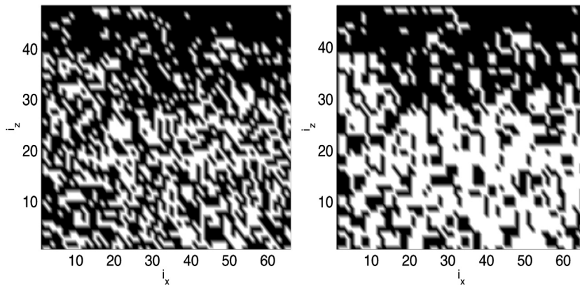
Fig. 9. Step 3-1. Database 1b. Conversion to the PIV mesh grid. Analysis from consecutive windows of 24 \times 24 pixels (left) and of 32 \times 32 pixels 2 (right). In each graph, the x - and y -axes correspond to the PIV mesh grid ( [i_x, i_z] \in [1 : n_x, 1 : n_z] = [66 \times 49] ).
