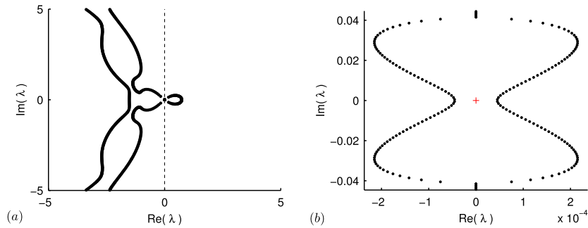
Fig. 2. In (a) and (b) we plot a numerical sampling of the (unstable) spectrum corresponding to the F \rightarrow \infty limiting spectral problems for the cases \alpha = -2 and \alpha > -2 , respectively, for a representative periodic stationary solution to the appropriate limiting profile equation.
