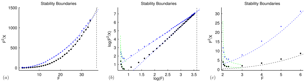
Fig. 1. Lower and upper stability boundaries for \nu = 0.1 , restricted to the slice q = 0.4F . Solid dots show numerically observed boundaries. Pale dashes indicate approximating curves given by (a) (upper) F^2/X = e^{0.087 F^{2.88}} and (lower) F^2/X = e^{-2.97 F^{2.83}} , (b) (upper) \log(F^2/X) = 2.88 \log(F) + 0.087 and (lower) \log(F^2/X) = 2.83 \log(F) - 2.97 . Pale dotted curves (green in color plates) indicate theoretical boundaries as F \rightarrow 2^+ . (c) Small- to large- F transition.
