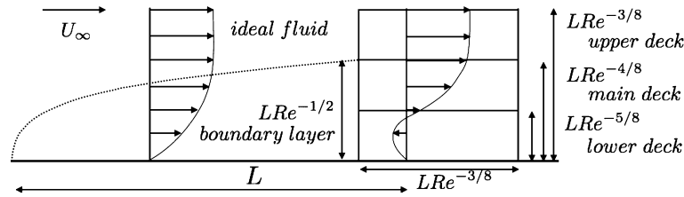
Fig. 1. Sketch of the flow of velocity U_\infty over a plate. If separation occurs at a position of characteristic length L , the boundary layer is of thickness LRe^{-1/2} at this length L . The triple-deck structure is of short length LRe^{-3/8} . Recirculation of the flow occurs near the wall in the lower deck of thickness LRe^{-5/8} .
