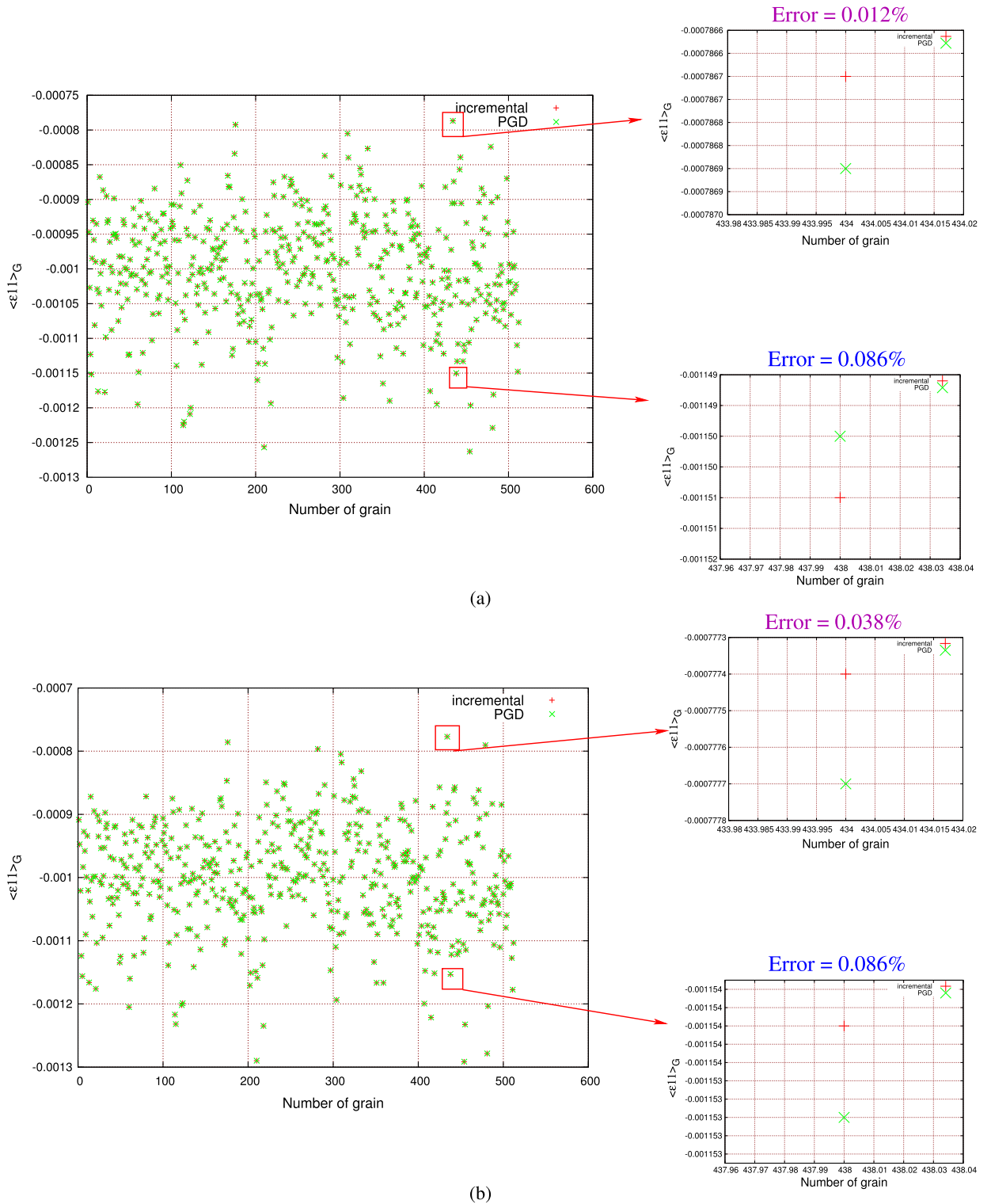
Fig. 10. Evolution of the error for the mesoscopic strain for two grains for incremental and PGD-V2 method for the (a) 10th loading cycle (b) 1000th loading cycle.
