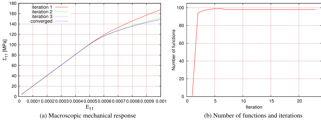
Fig. 5. Convergence of the PGD-V1 method.
