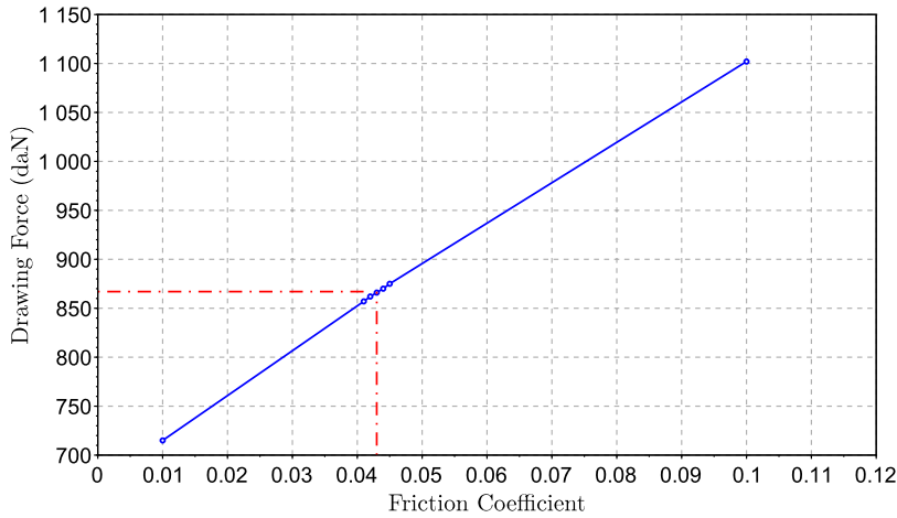
Fig. 5. Drawing force evolution as a function of the friction coefficient \mu_{\text{tube}/\text{die}} (tube sinking case).
