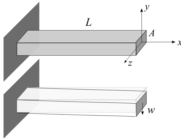
Figure 1. Free vibration test: the cantilever beam is subjected to an initial vertical displacement at x = L and then let go.
