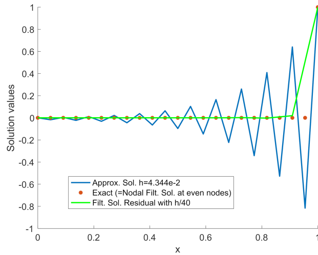
Figure 5. Residual-based “a posteriori VMS”. Filtered solution obtained with initial values for the parameters yielding the optimal nodal values \alpha_i^{nb} for the gradient method. The filtered solution approaches values very close to those of the exact solution at even grid nodes, when the residual is computed with a fine enough grid.
