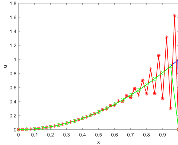
Figure 3. Test 1. Exact solution (line marked by +) of the convection-diffusion equation with linear source term and homogeneous boundary conditions, approximation by FEM Galerkin \mathbb{P}_1 (line marked by *) and nodal “a posteriori VMS” filtering (line marked by o), for Pe_h = 10 .
