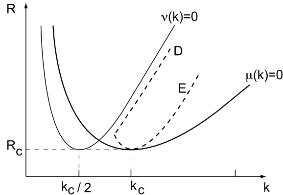
Figure 2. Neutral stability curves \mu(k) = 0 for the mode of wave number k and v(k) = 0 for the mode of wave number 2k . The domain of stable stationary patterns is limited by the Eckhaus instability (E) and the drift bifurcation (D).
