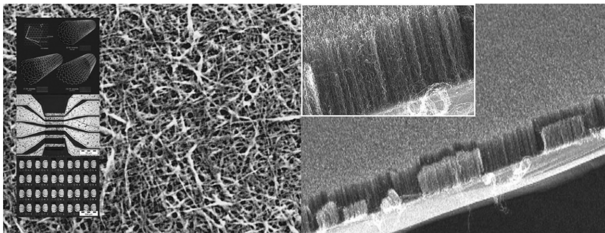
Scanning Electron Microscope images of structured carbon nanotubes or nanotubes grown as a carpet. Insert: Opto-electronic devices based on carbon nanotubes (ONERA/DOTA and CNRS/LPN). The image on the right is published with permission from RDDC Valcartier
