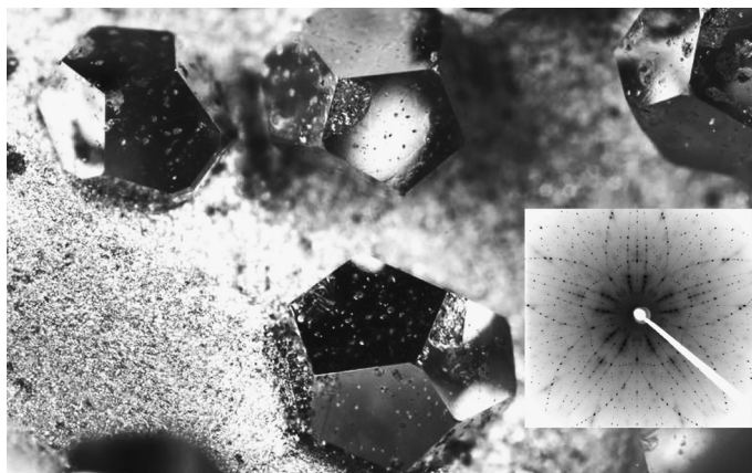
i-CdRE (RE = Gd, HO, Tm) monoquasicrystals (Photo : A.P. Tsai and coworkers, Tohoku University, Japan). Insert: Laue XRD diagram of i-AlPdMn around a quinary direction, recorded by the team of W. Steurer (Zurich, Switzerland).
