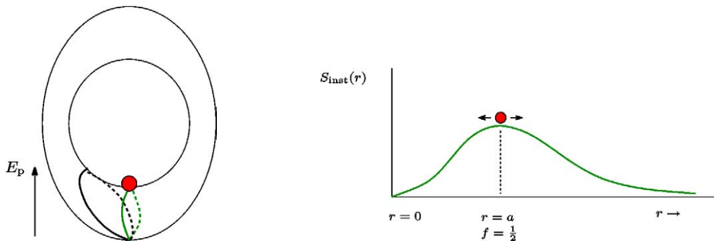
Fig. 1. The picture on the left shows in a schematic way the existence of a non-contractible loop in configuration space, as well as the presence of the sphaleron (large dot) at the saddle point. The picture on the right shows the action density S(r) of the instanton in the Euclidean theory, together with the special configuration at r = a which is used to construct the sphaleronic particle in the Lorentzian theory.
