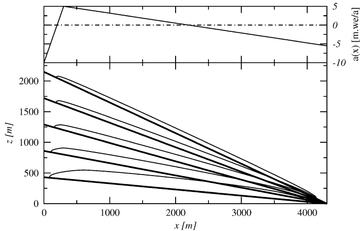
Fig. 3. Geometry of the glacier as given by the SIA formulation for the five bedrock slopes from \alpha = 0.1 to \alpha = 0.5 by steps of 0.1 and for an accumulation parameter a_0 = 5.0 m.w.e. a^{-1} whose corresponding spatial distribution is also shown (upper part).
