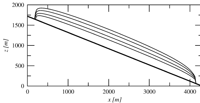
Fig. 4. Geometry of the glacier given by the SIA formulation for the four maximal accumulation a_0 = 0.1 , a_0 = 0.5 , a_0 = 2.0 and a_0 = 5.0 m.w.e. a^{-1} and for a bedrock slope \alpha = 0.4 . For a better reading, the ice thickness has been enlarged 5 times. The larger the a_0 value, the thicker the ice.
